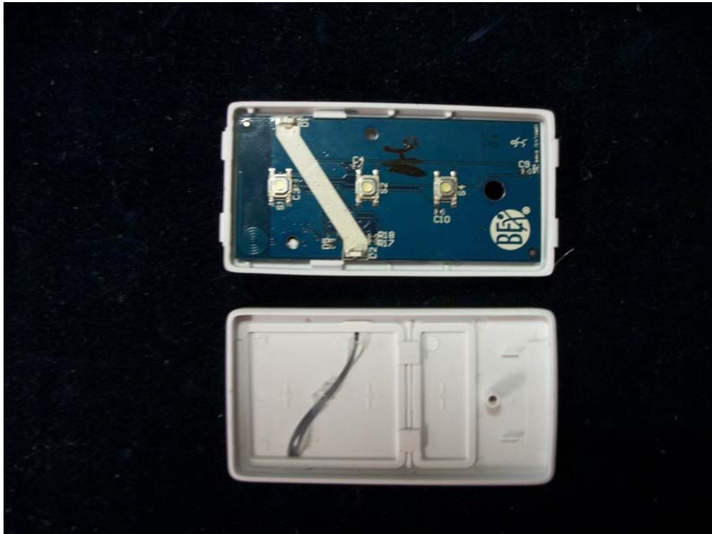
7.3 Inside View
