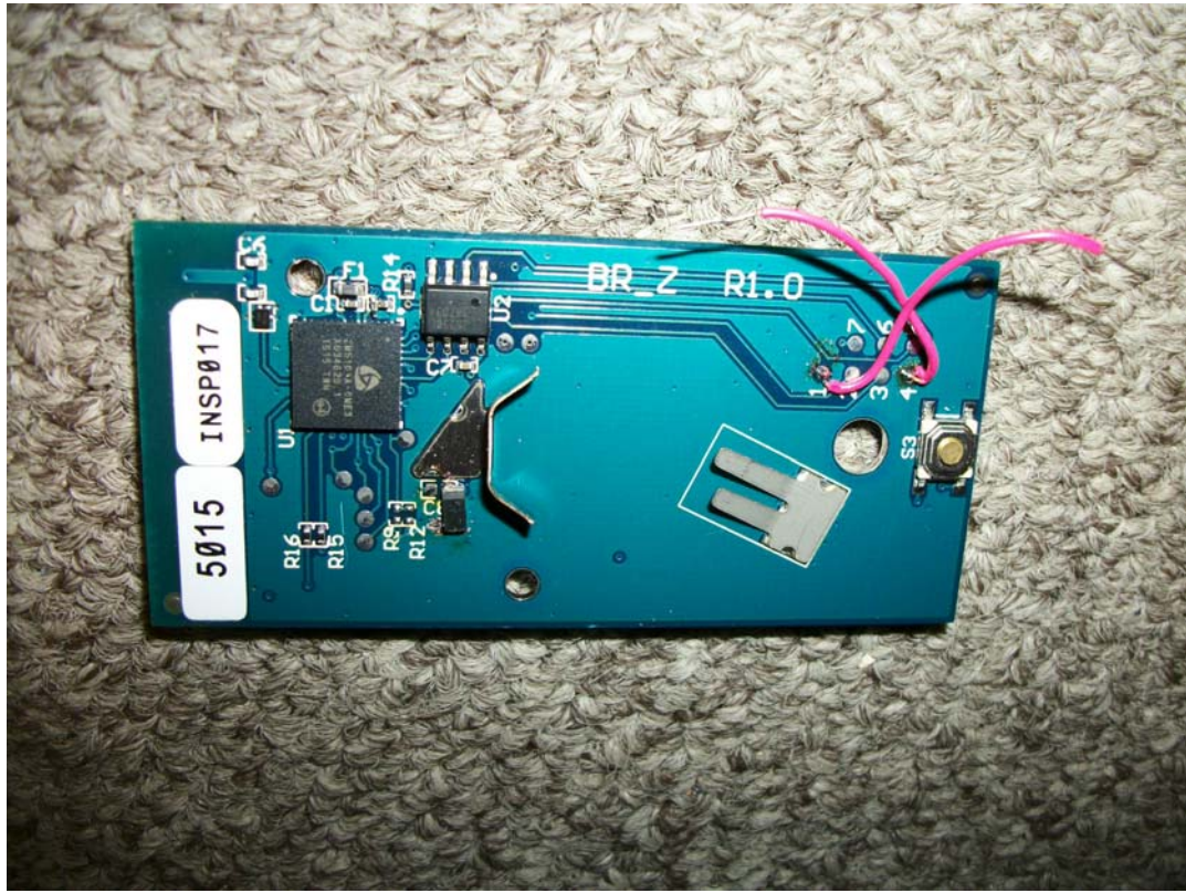
7.4 Components View
