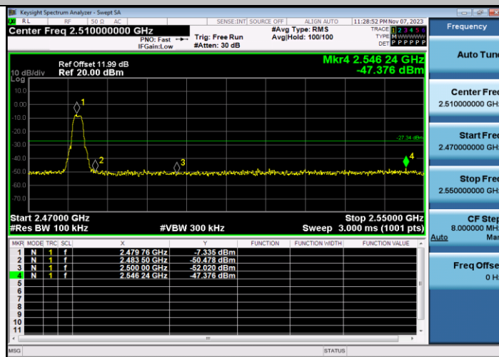
Zigbee_1M_Ant1_High_2480
