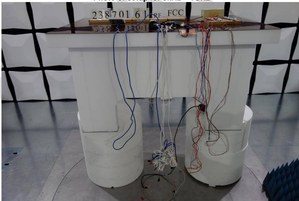
Photo of test setup 1GHz – 40GHz
