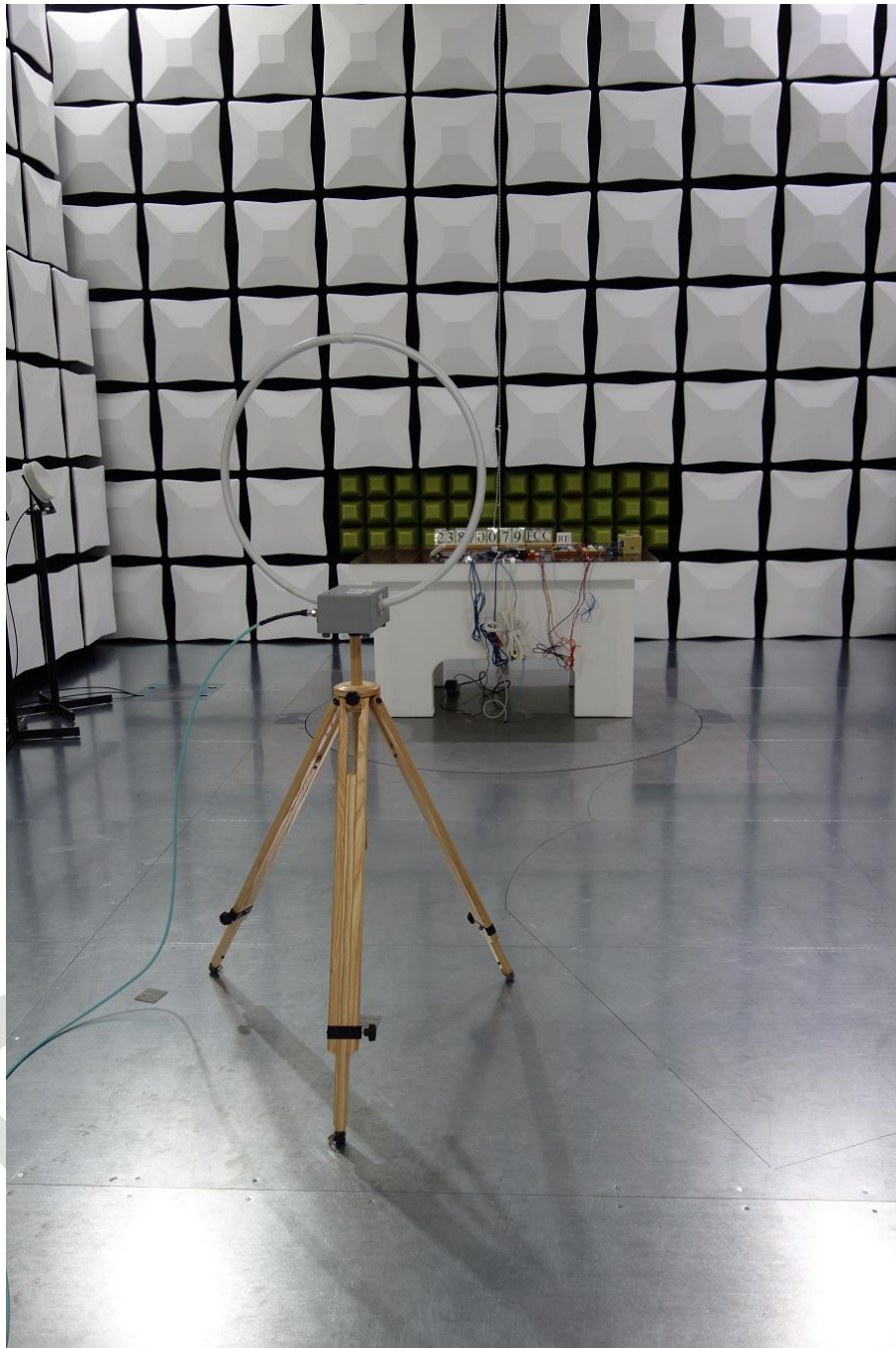
Photo of test setup for 9kHz – 30MHz parallel position
