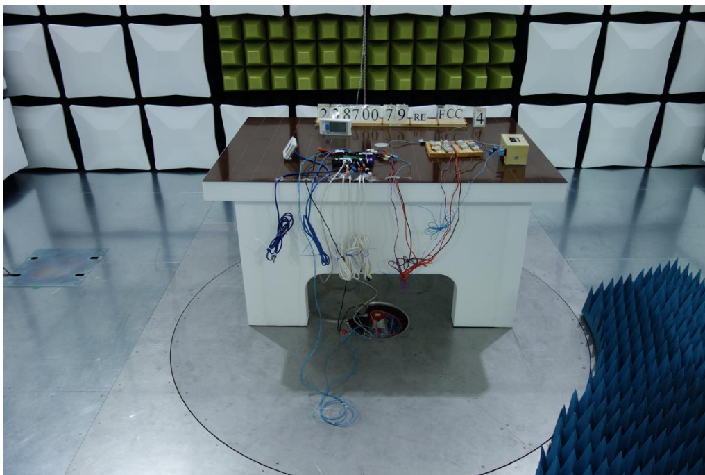
Photo of setup for 9kHz – 1GHz
