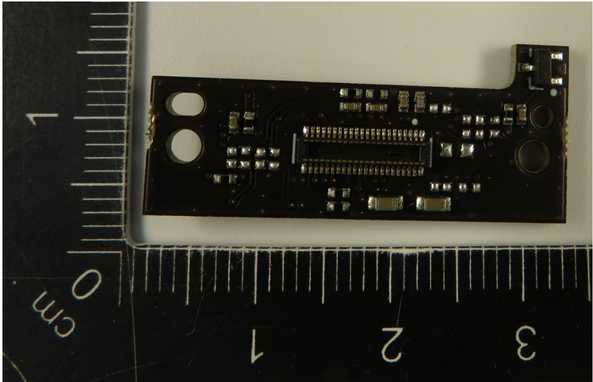
PCB 2 bottom:
