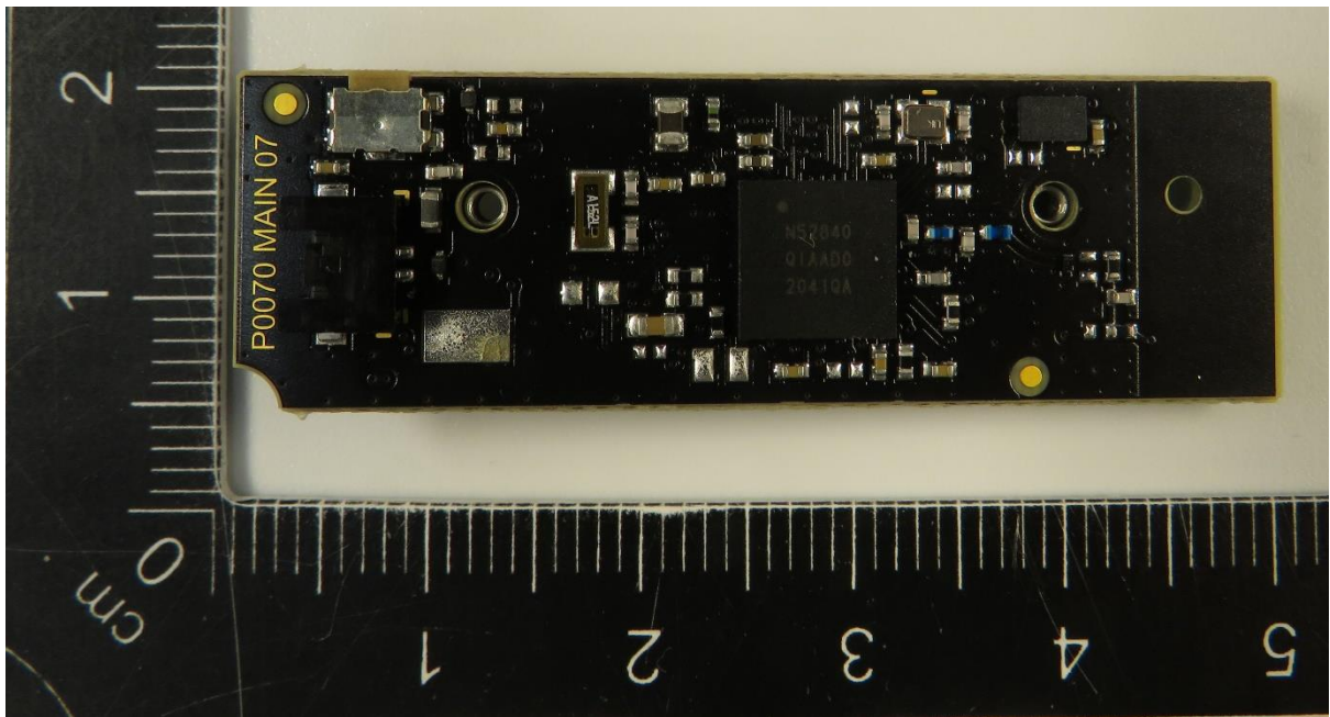
Main PCB Top
