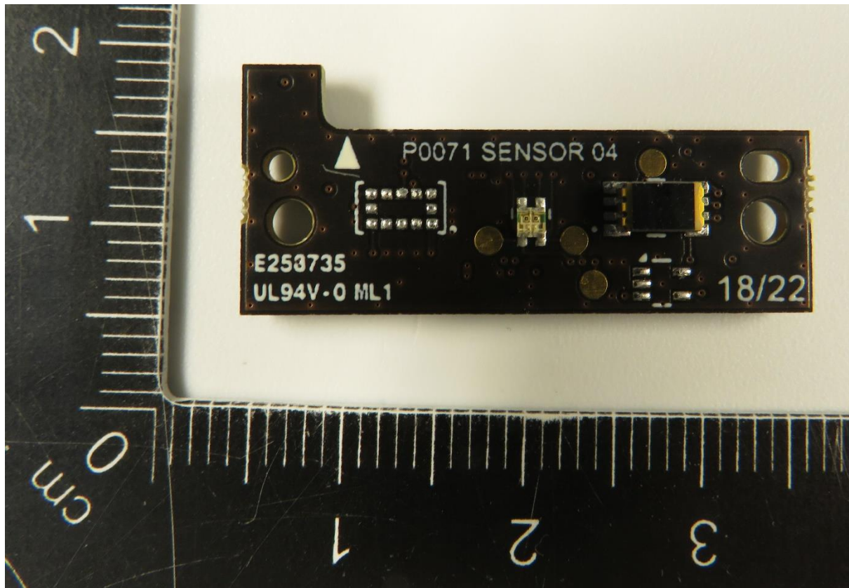
PCB 2 top:
