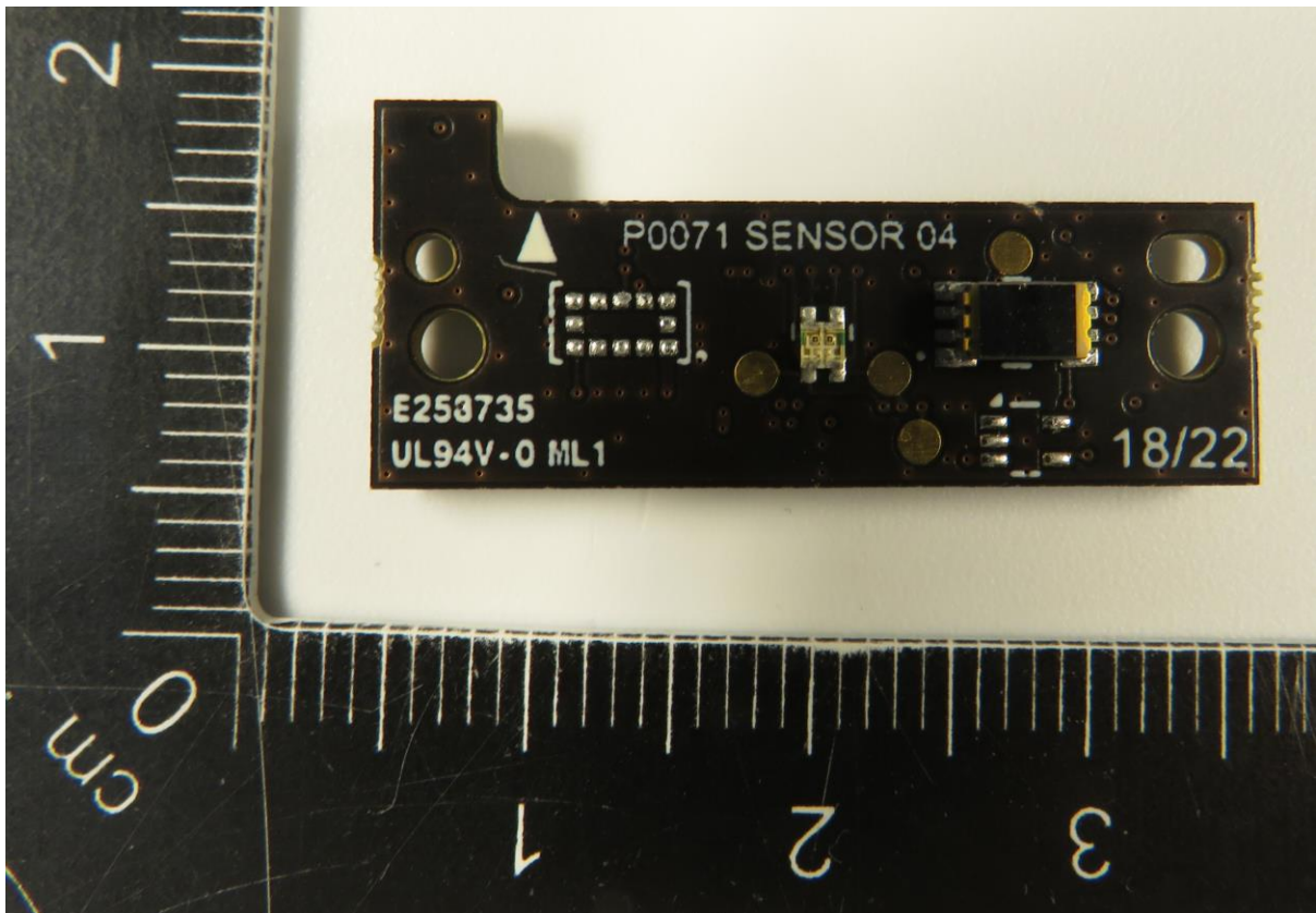
PCB 2 top:
