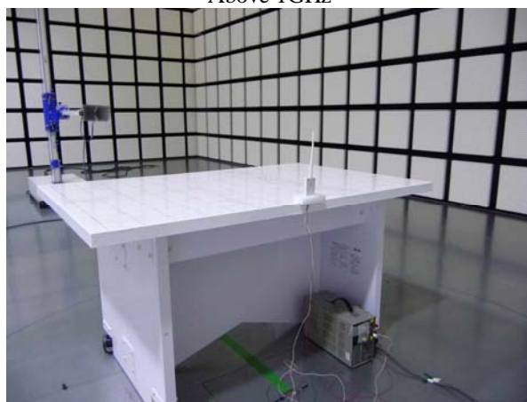
Above 1GHz
