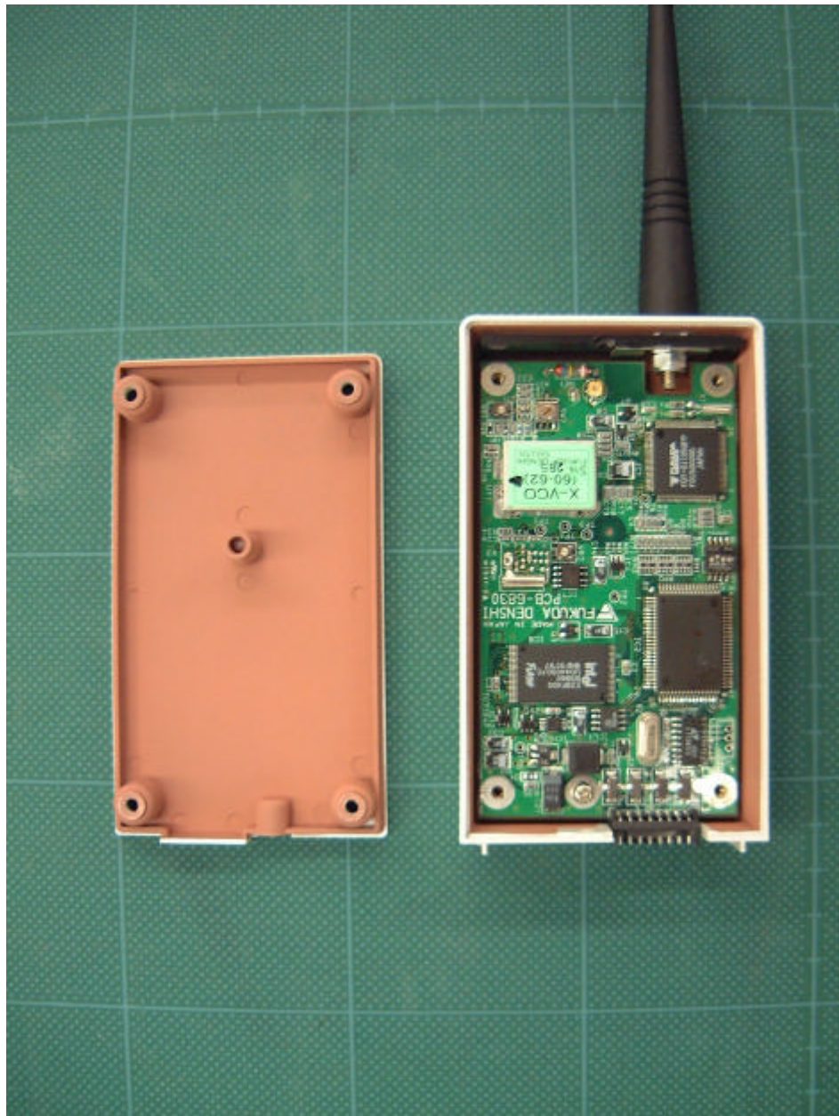
PCB Component Side
