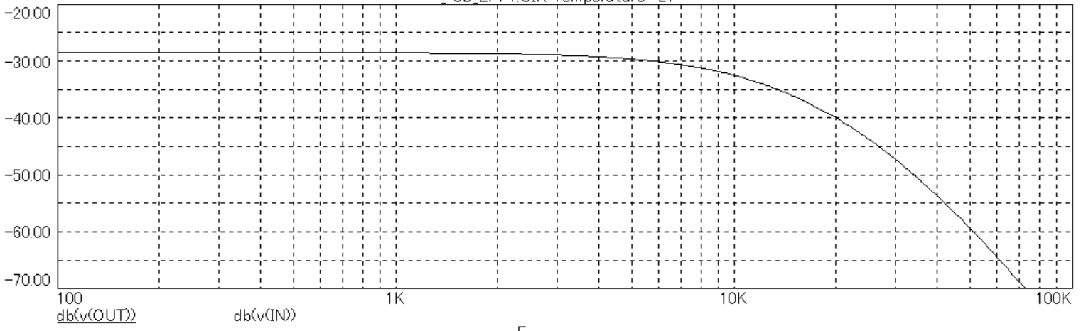
SD_LPF1.CIR Temperature= 27
