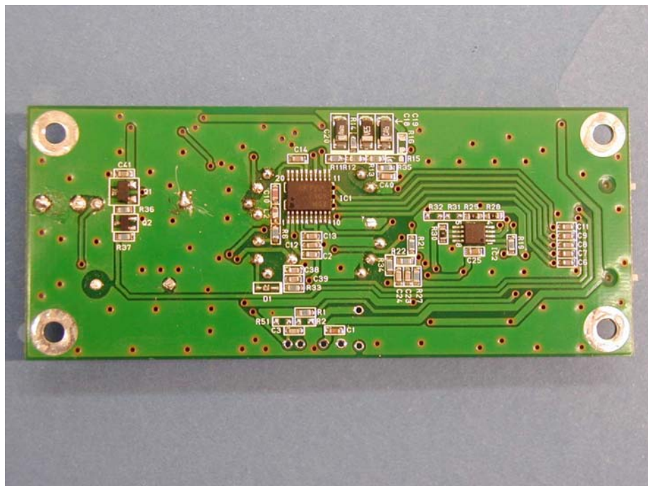
Back of Radio Module
