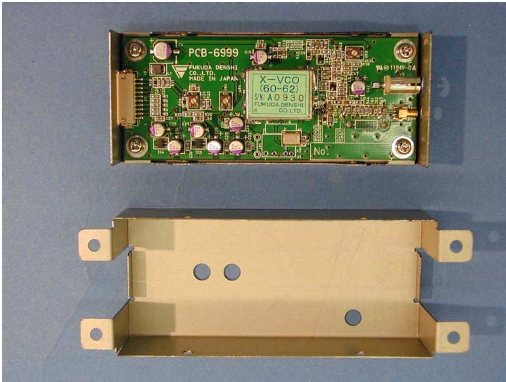
RF module and Shield Cover
