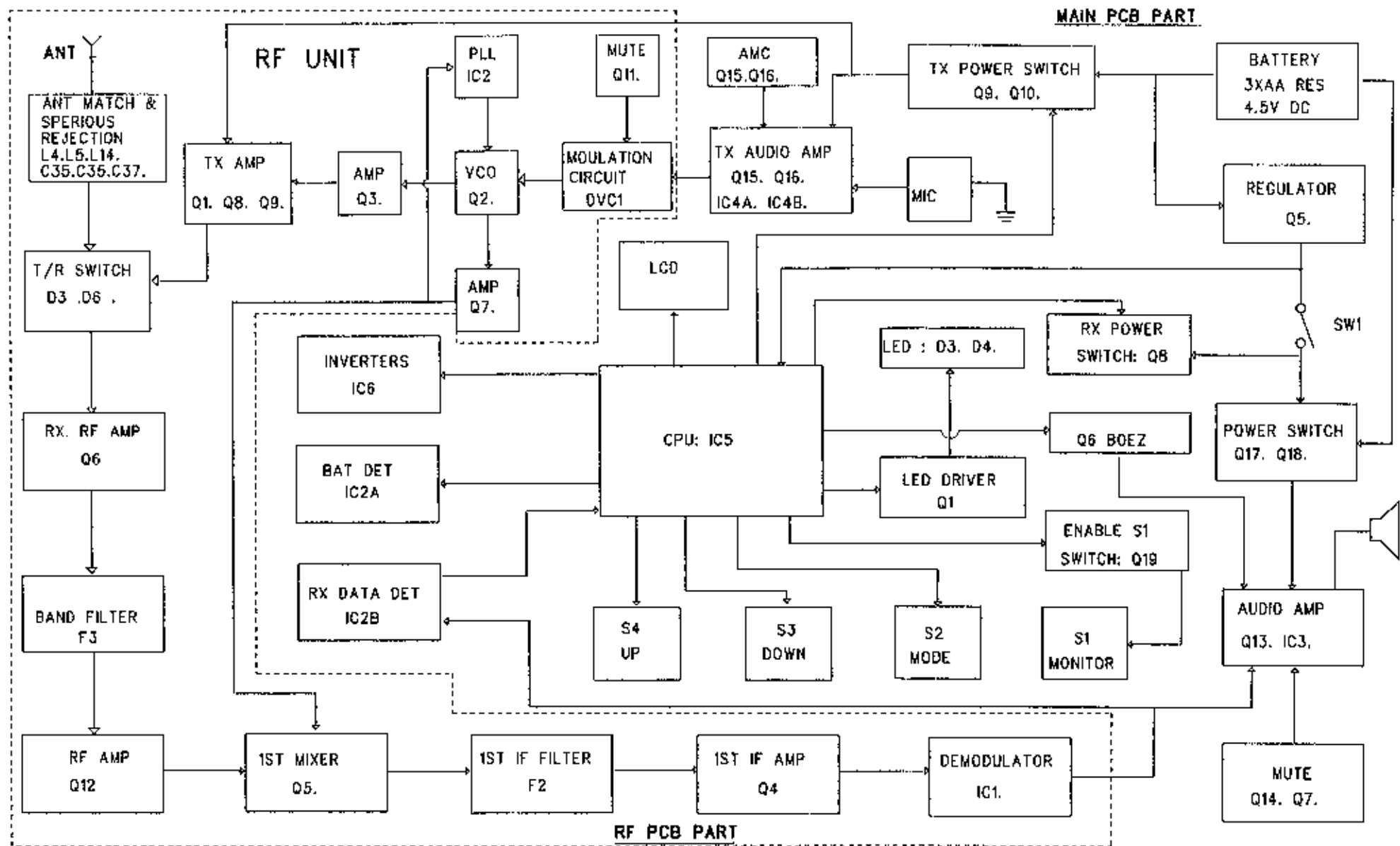
BLOCK DIAGRAM (FRS-0128)
