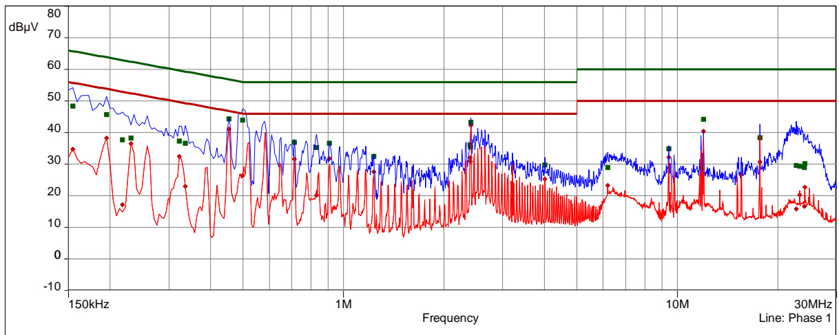
CISPR 22/CISPR22B
