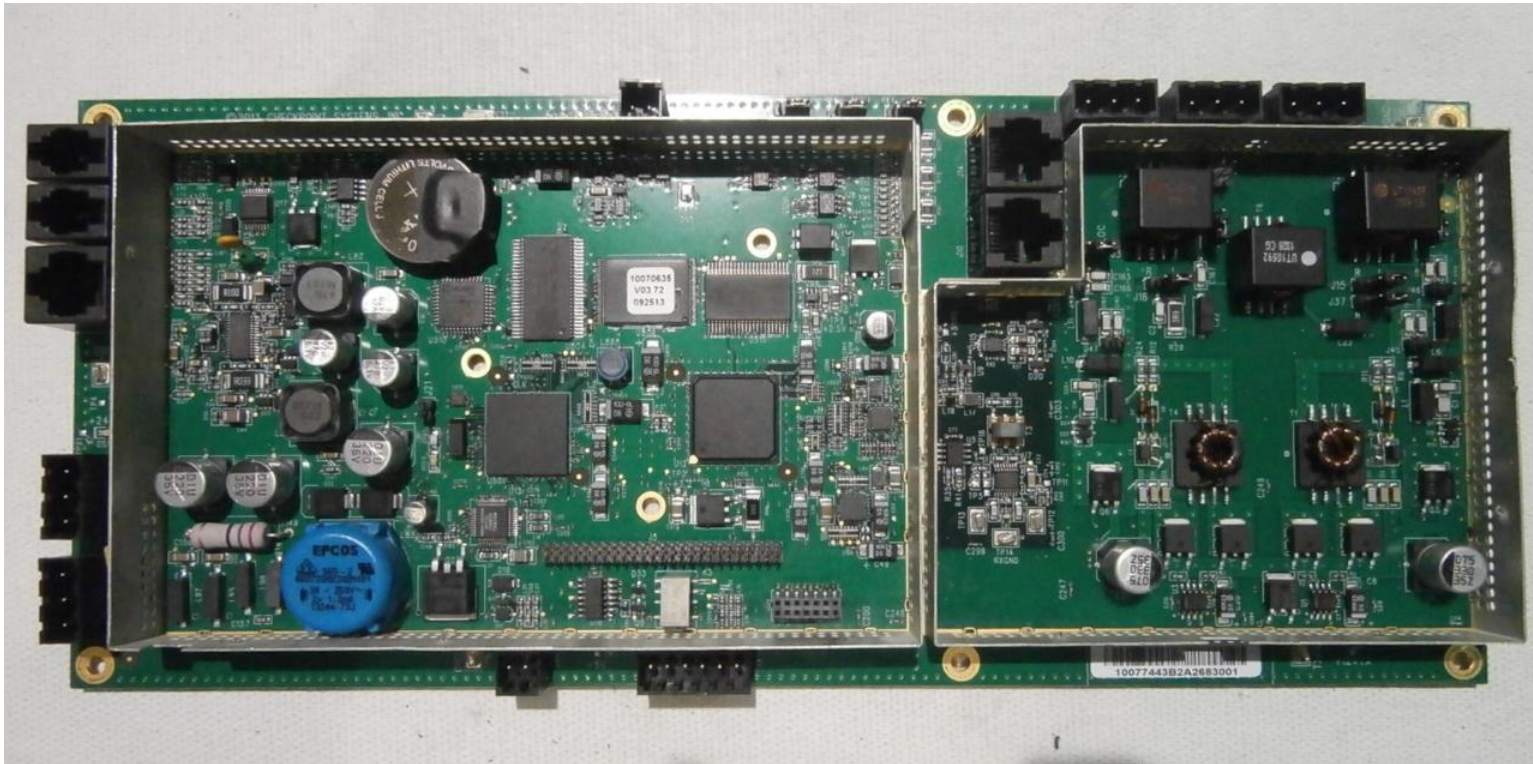
Top Module without Shielding and Daughter Board Removed
