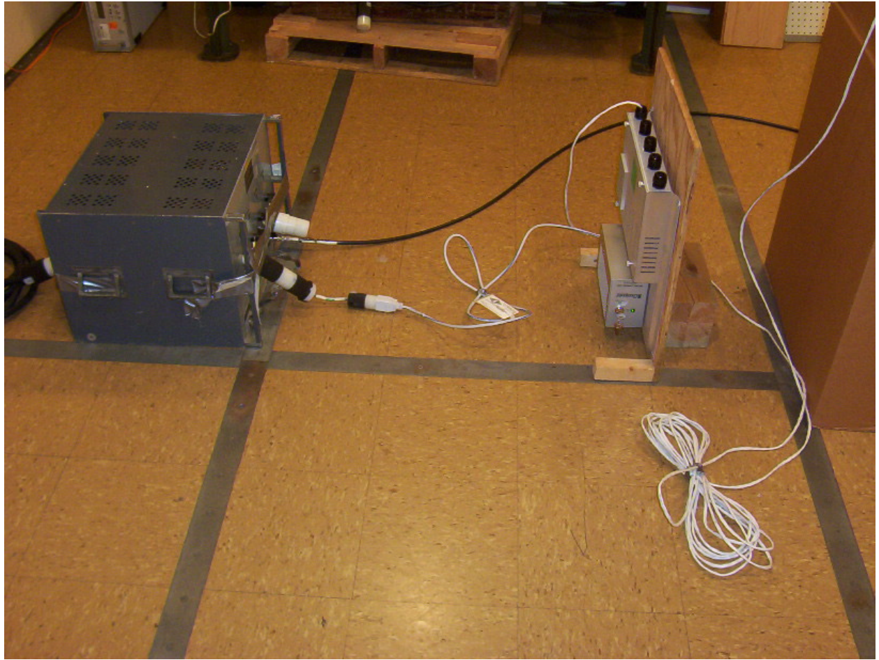
Photo 2 – Detail of LISN to Controller Arrangement
