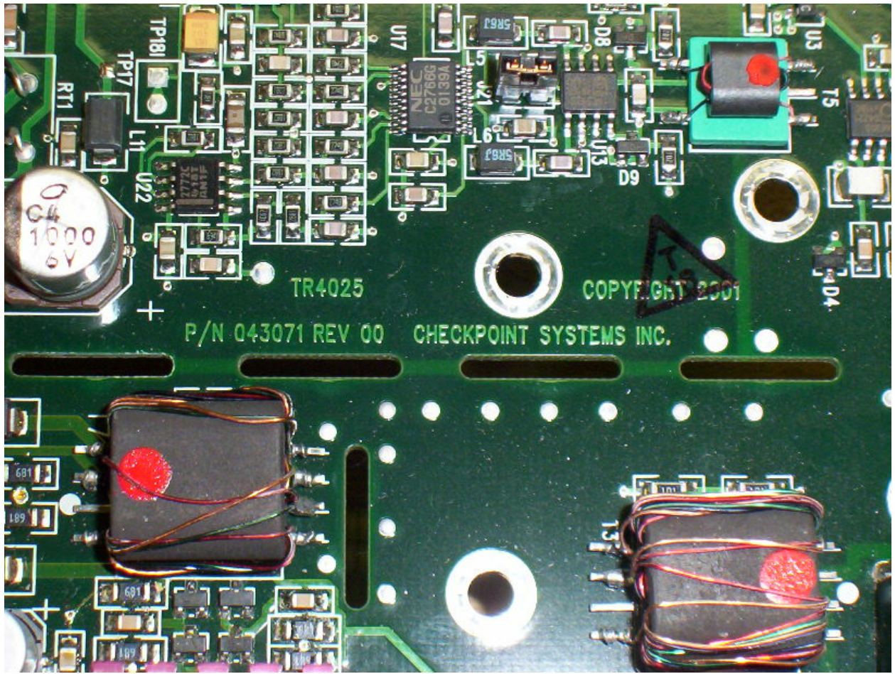
Photo 3 – View of Labeling on TR4025 Control PCB
