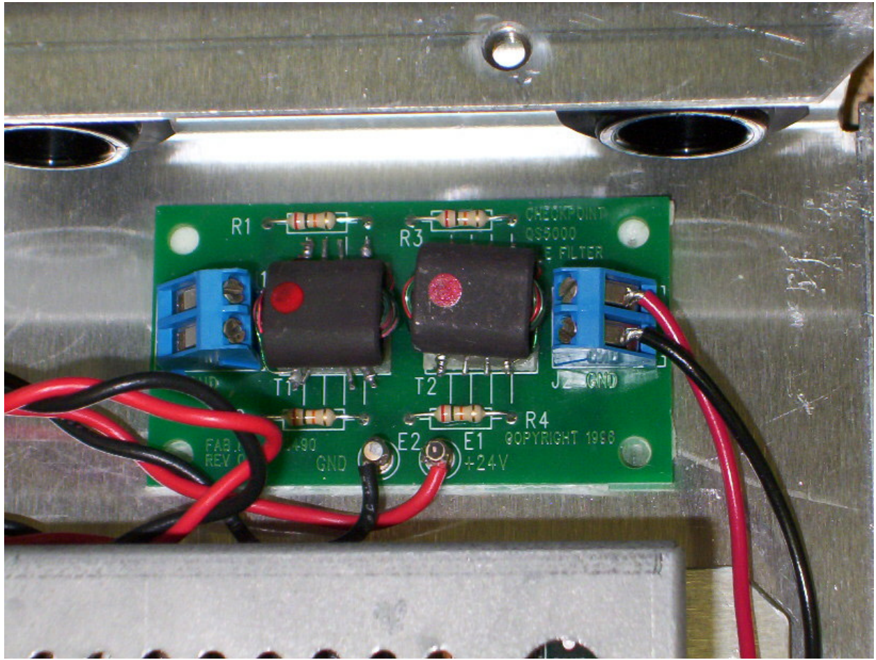
Photo 1 – Top View of DC Filter Board
