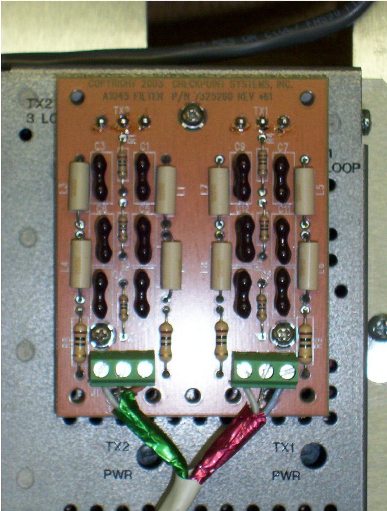
Photo 2 – Top View of Antenna Matching Board
