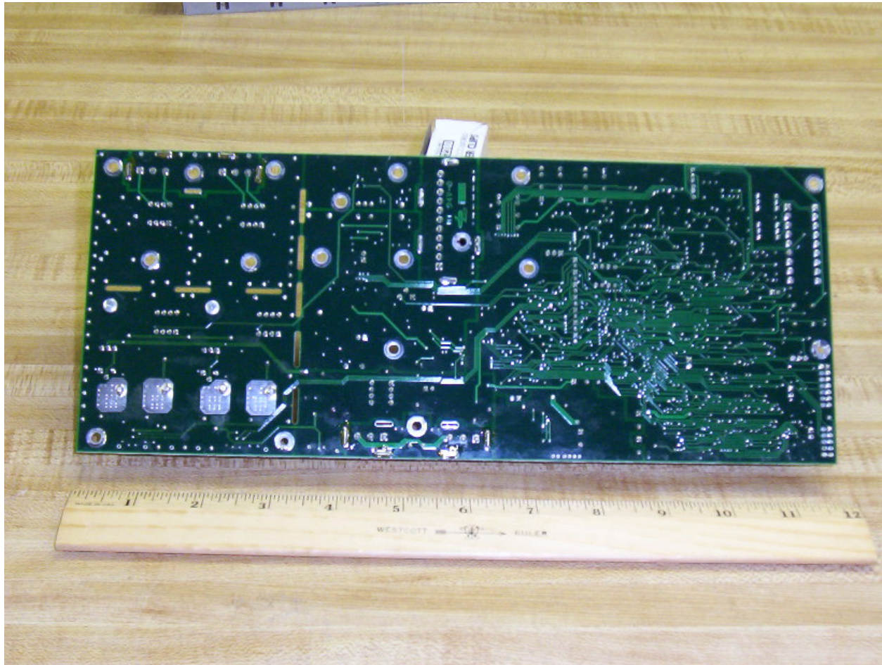
Photo 2 – Bottom Side of TR4025 Control PCB
