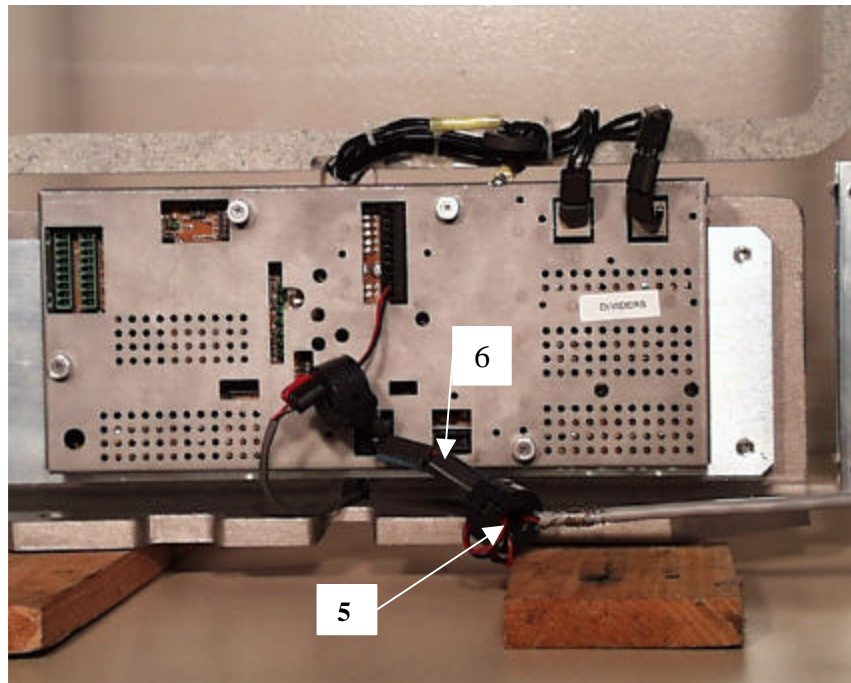
Photo 3 – Ferrite Locations
