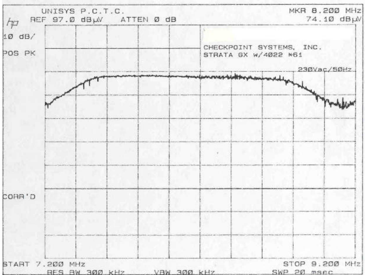
Photo 6 – Bandwidth Plot
