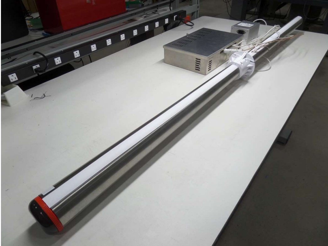
Figure 1: NS40 antenna, Neo Remote Electronics Controller, power supply
