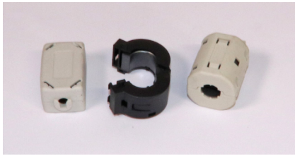
Figure 4: Common Ferrites
