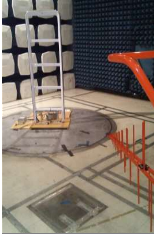
Photograph 3. Radiated Emissions, NP10 and NP20, Below 1 GHz
