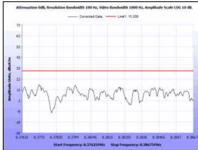
Plot 42. Radiated Restricted Band Edge, NP10, 8.37625 MHz – 8.38675 MHz
