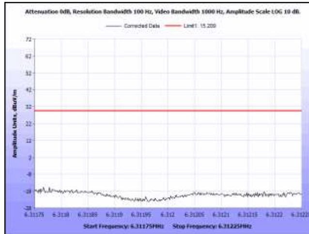
Plot 39. Radiated Restricted Band Edge, NP10, 6.31175 MHz – 6.31225 MHz
