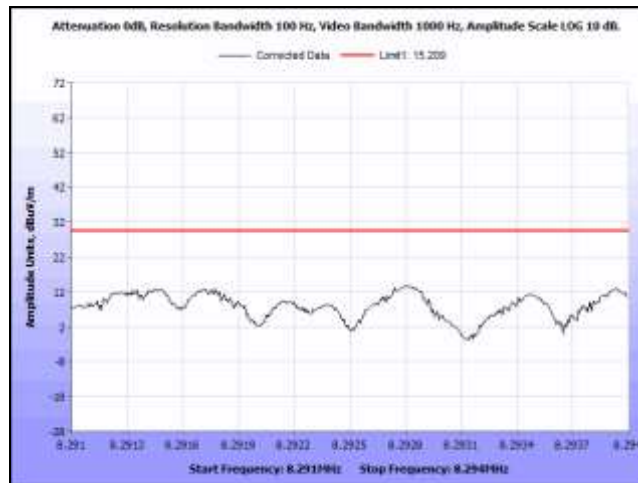
Plot 40. Radiated Restricted Band Edge, NP10, 8.291 MHz – 8.294 MHz
