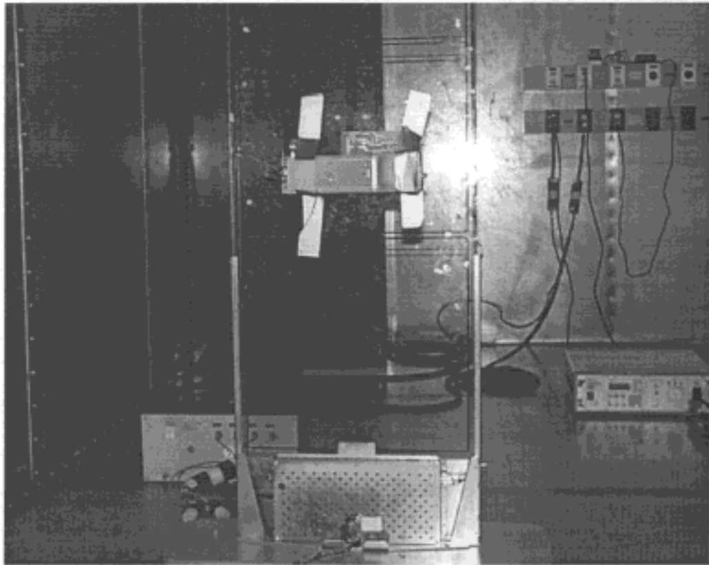
Long Range Reader - Conducted EMI Test Setup (plastic skins removed)
