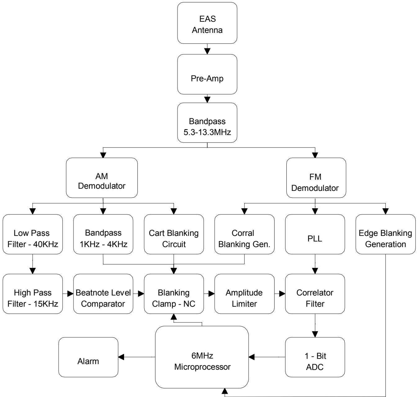
FIGURE 1 R3520 BLOCK DIAGRAM
