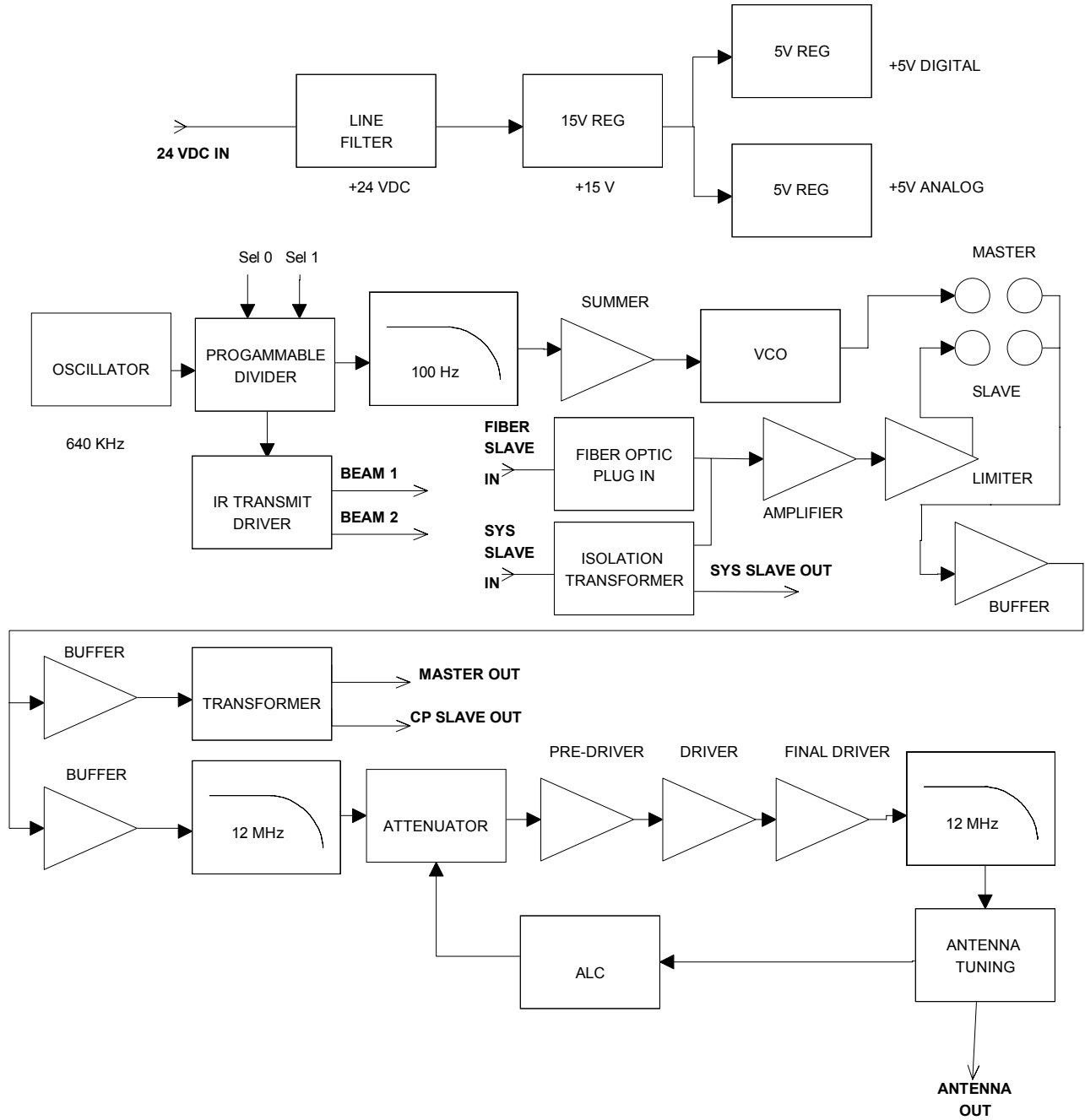
Figure 1 T3600 BLOCK DIAGRAM
