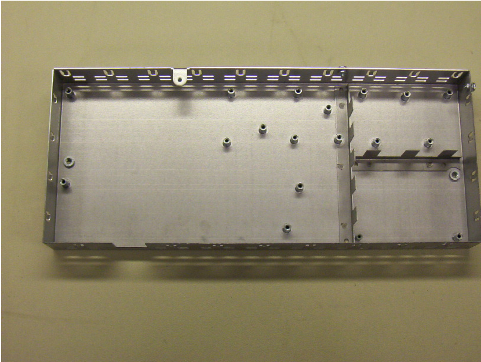
PHOTO 6 – INSIDE OF CONTROL MODULE HOUSING WITH PCB REMOVED
