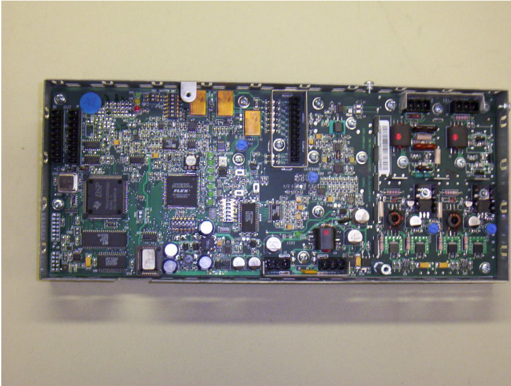
PHOTO 5 – VIEW OF CONTROL PCB MOUNTING IN HOUSING
