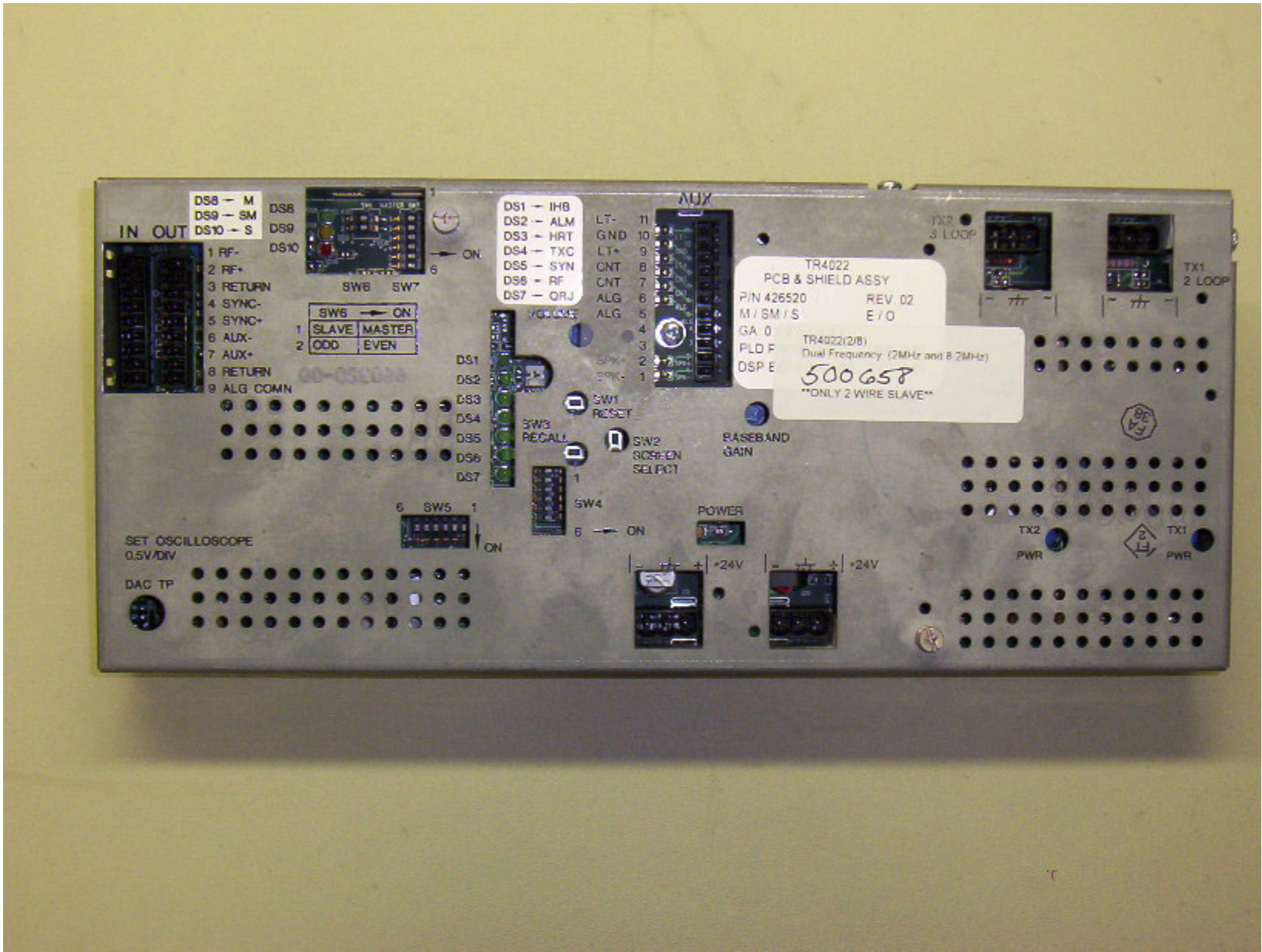
PHOTO 2 – TOP VIEW OF LIBERTY DX CONTROL MODULE HOUSING
