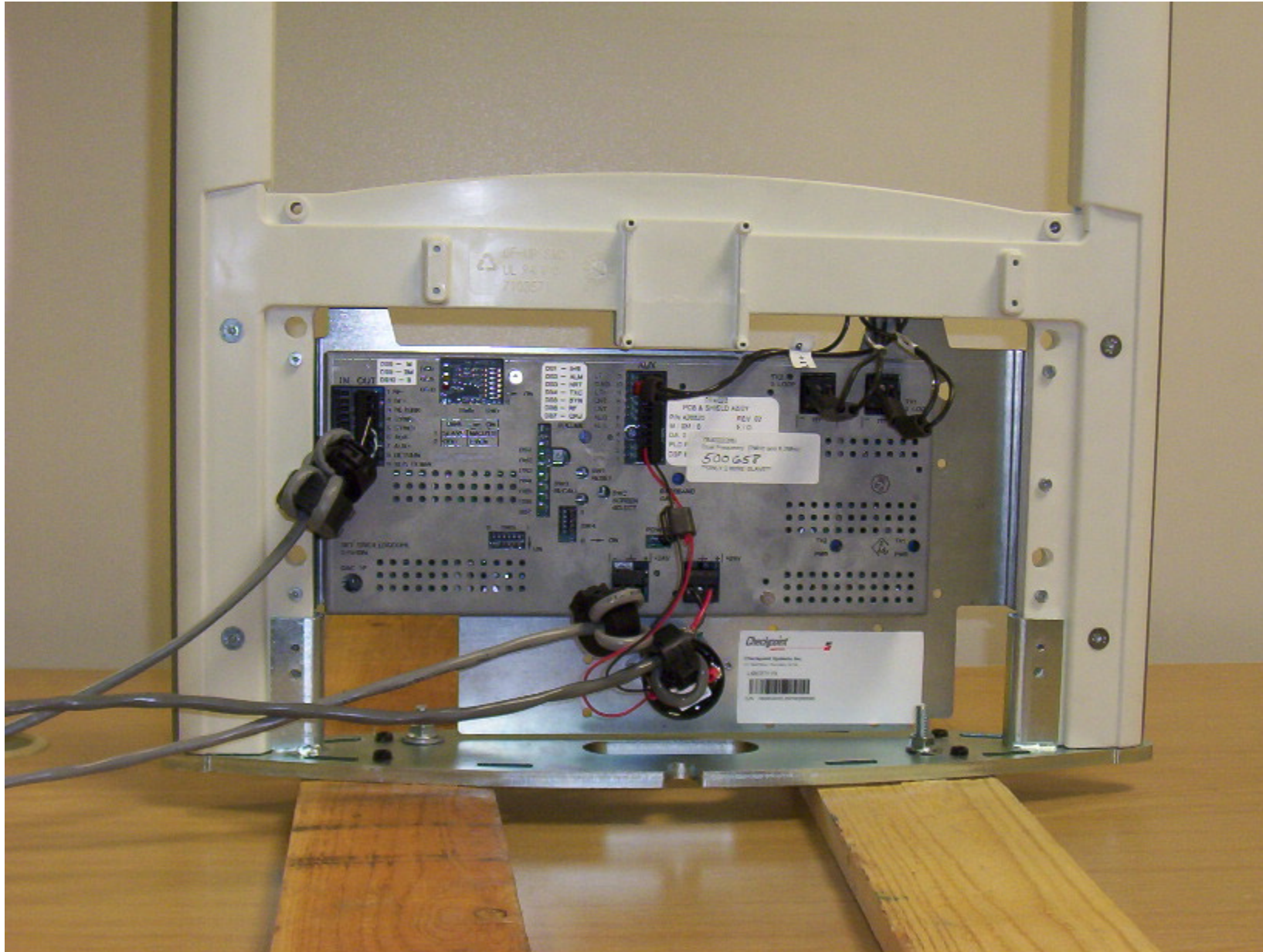
PHOTO 1 – LOWER DETAIL OF LIBERTY DX WITH EXTERNAL DRESS COVER REMOVED
