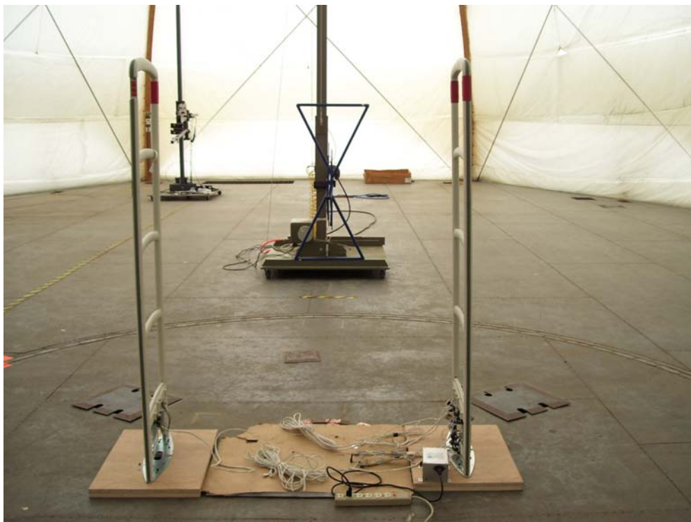
Figure 3 – Final Radiated Emissions at OATS site (rear view)
