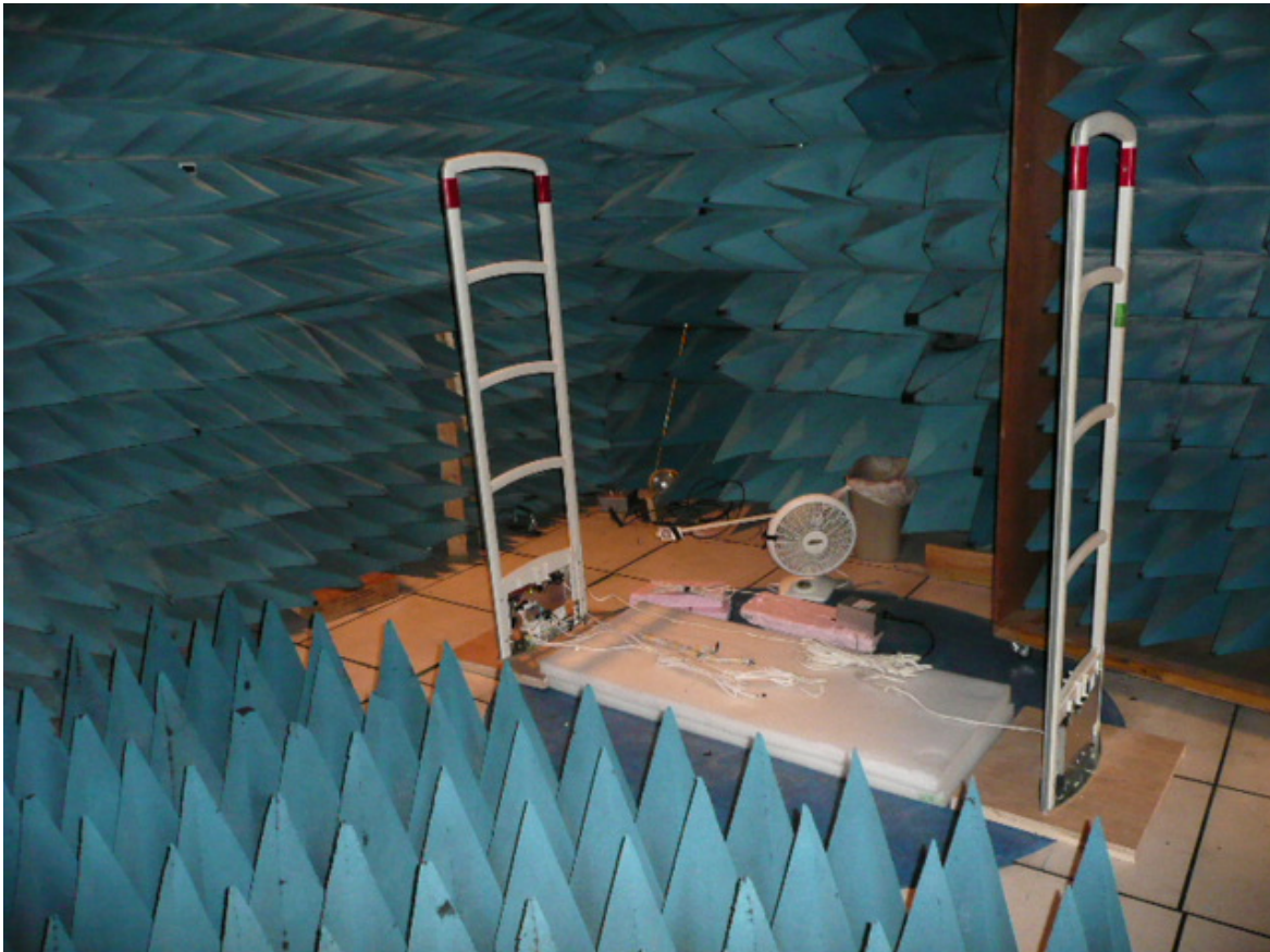
Figure 1 – Prescans in semi anechoic chamber
