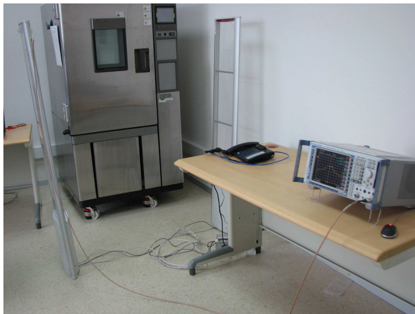
Photograph 4: Set-up for emission bandwidth & duty cycle
