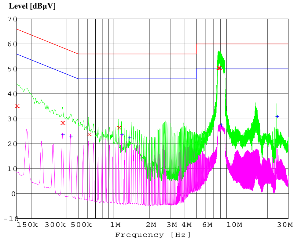
Figure 2: Spectral diagram, conducted emission, 150kHz - 30MHz, N (PX)
