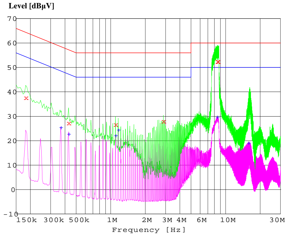
Figure 4: Spectral diagram, conducted emission, 150kHz - 30MHz, N (QX)
