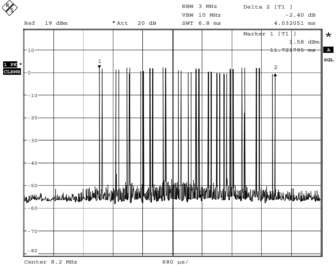
Figure 6: Duty cycle measurement result
