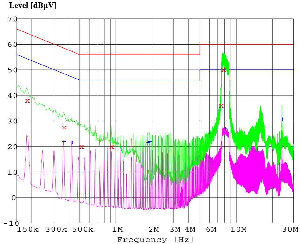
Figure 1: Spectral diagram, conducted emission, 150kHz - 30MHz, L (PX)
