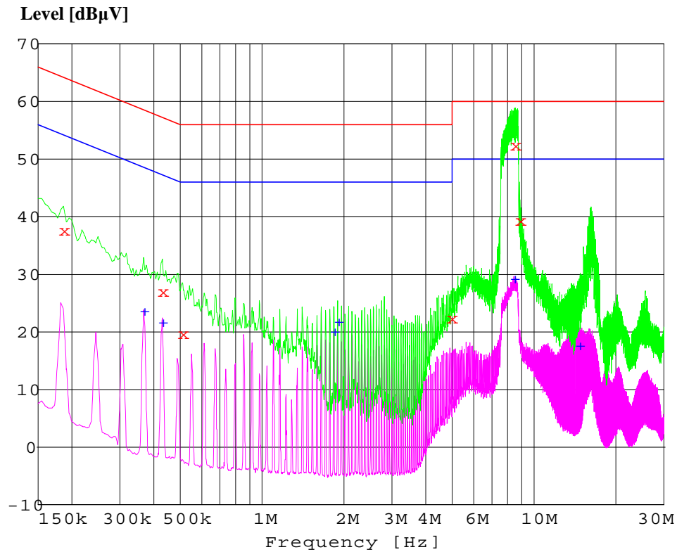
Figure 3: Spectral diagram, conducted emission, 150kHz - 30MHz, L (QX)
