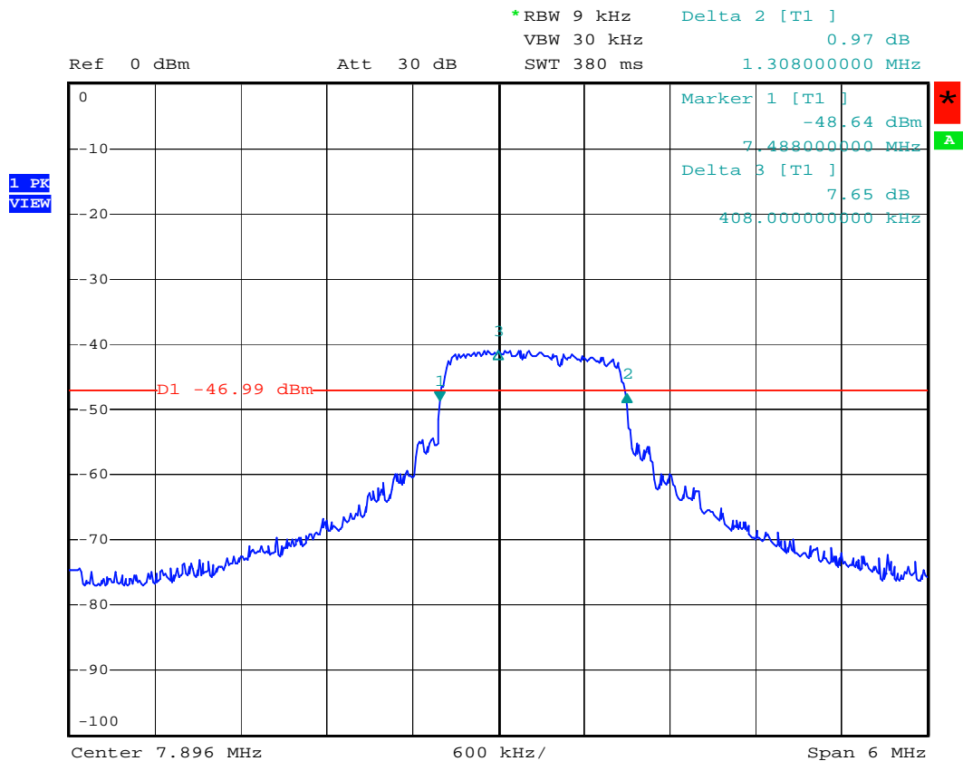
Figure 5: Spectral diagram, emission bandwidth measurement
