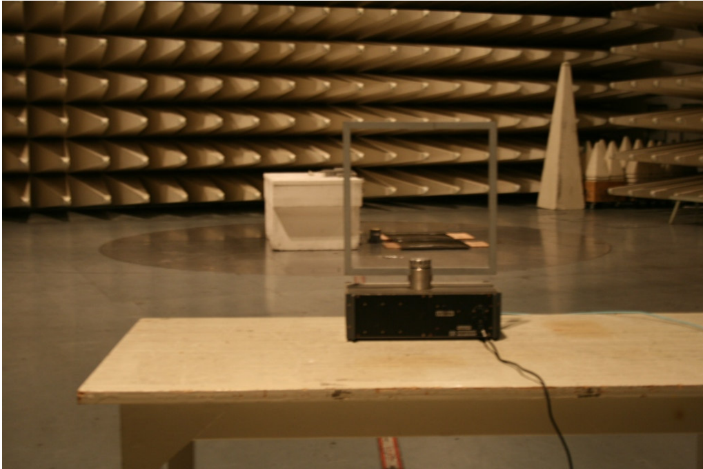
With 6 foot shielded product
