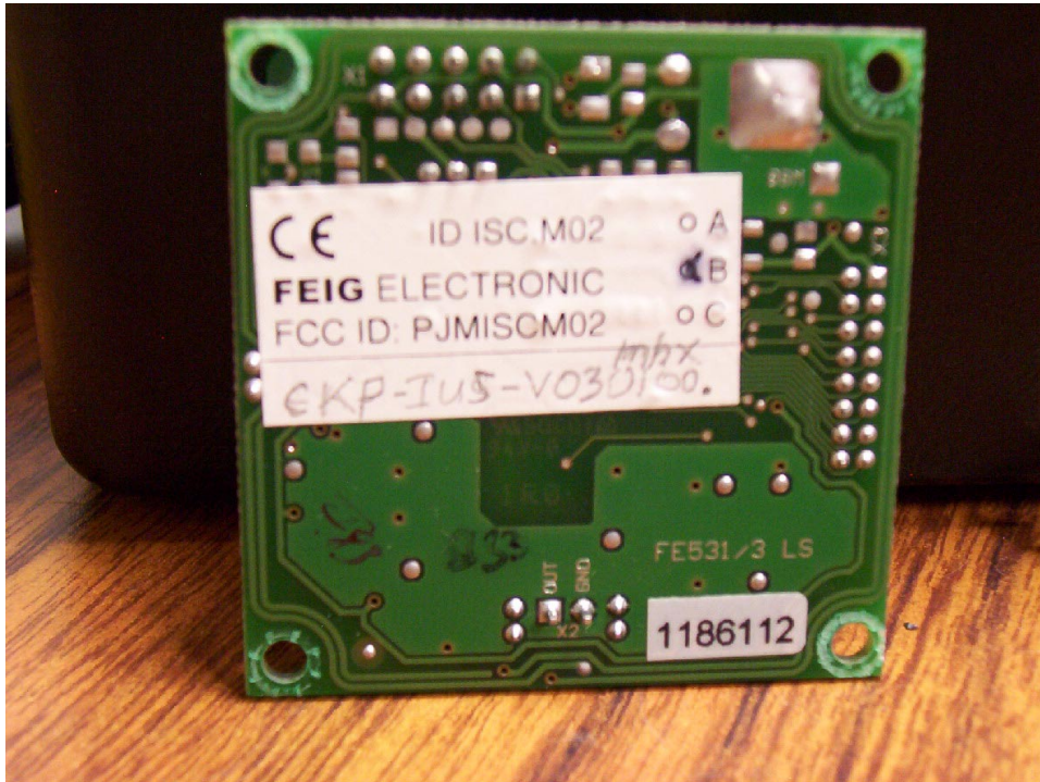
FEIG Transmitter PCB (Solder Side)
