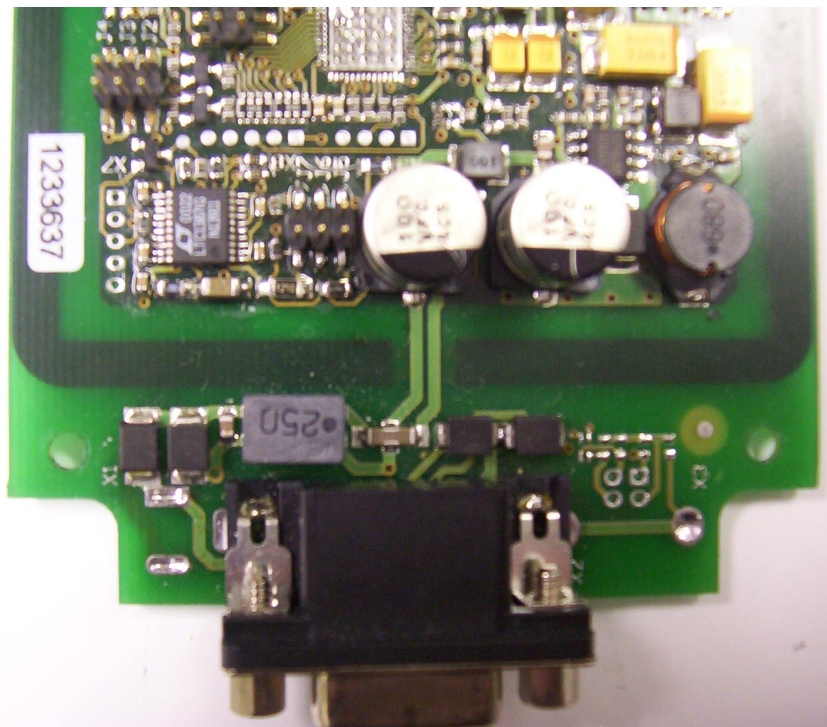
Transmitter PCB top 2
