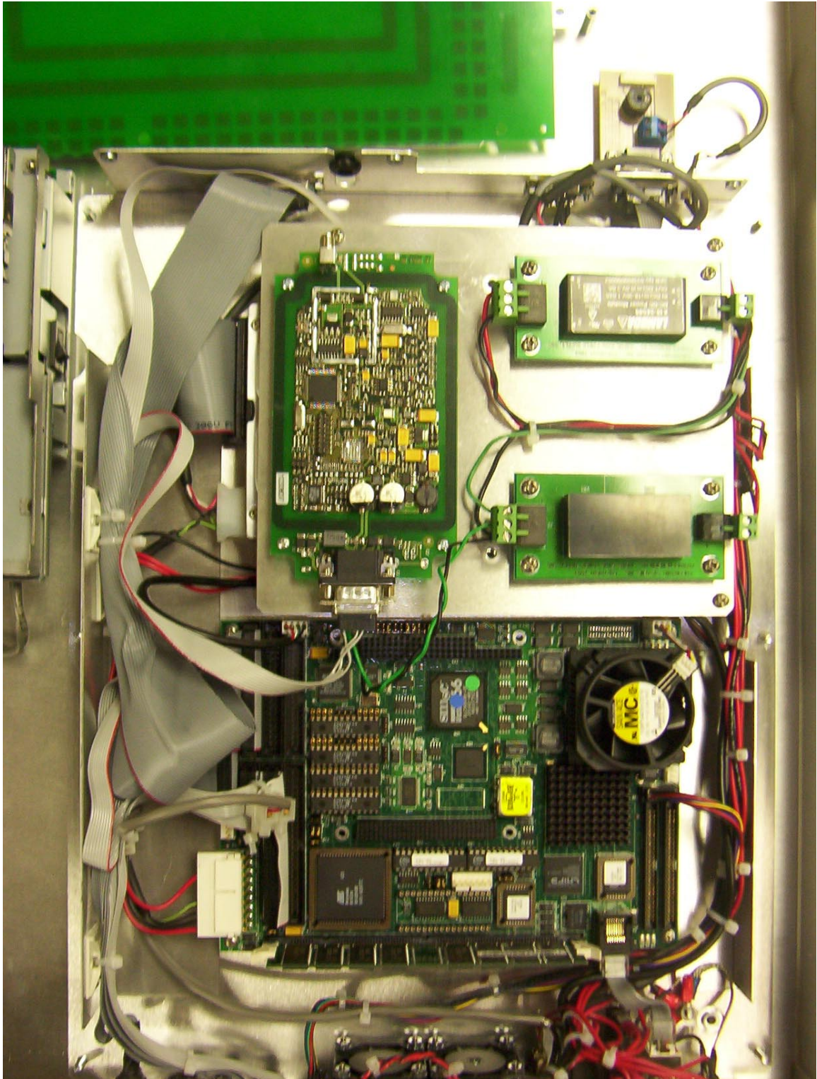
SBC, Transmitter and DC power module location
