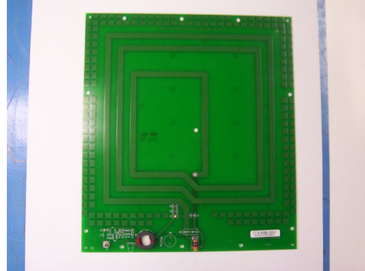
Antenna PCB top
