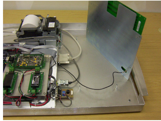
Antenna assembly
