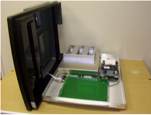
Cover Opened
