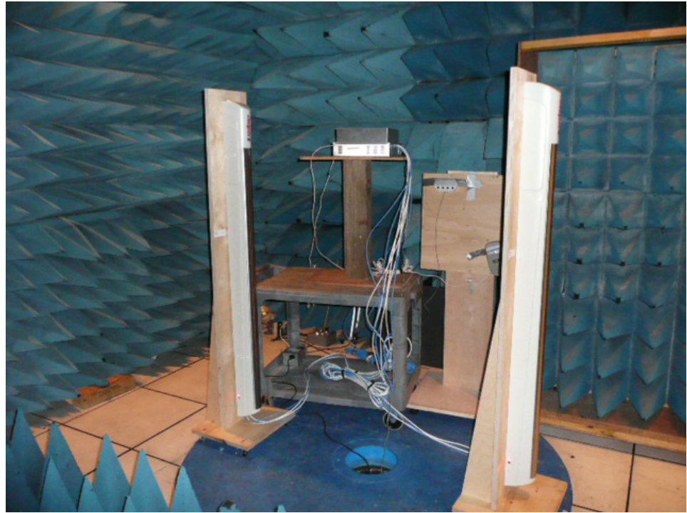
Radiated Spurious Emissions Pre-scan Configuration 1
