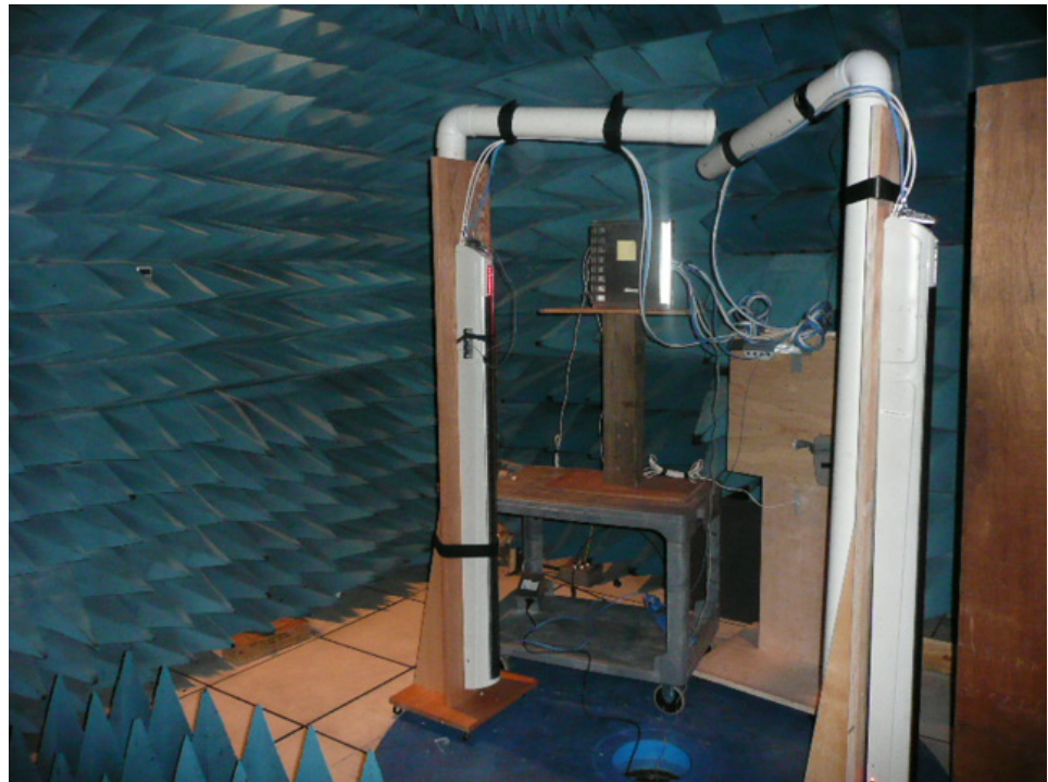
Radiated Spurious Emissions Pre-scan Configuration 2
