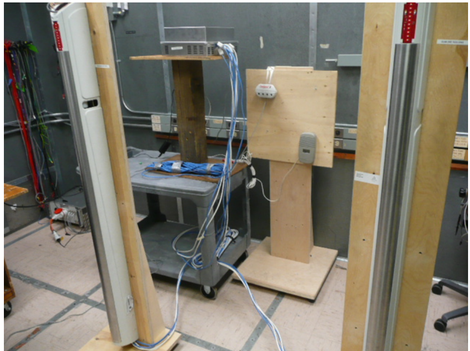
Conducted Emissions Measurement Configuration 1
