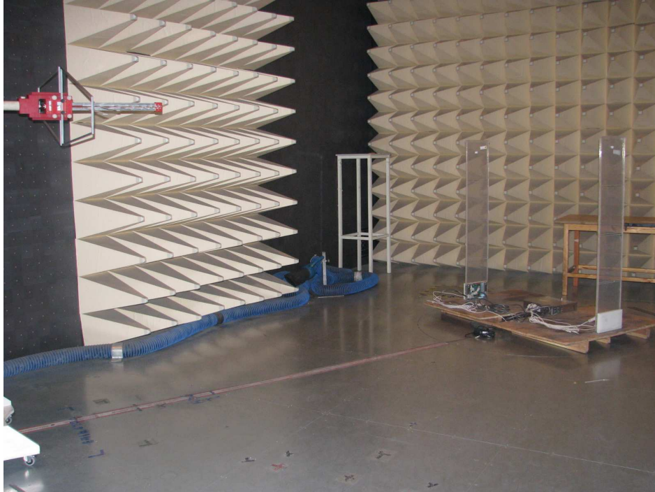
Photograph 3: Set-up for radiated emission (30 - 1000MHz)
