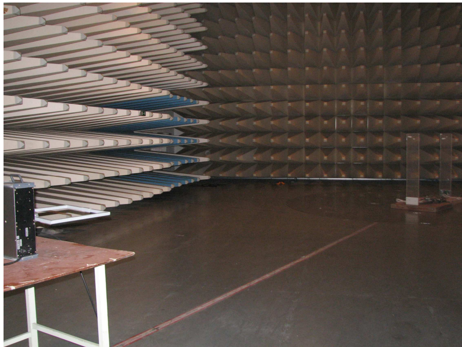
Photograph 2: Set-up for radiated emission (9kHz - 30MHz)
