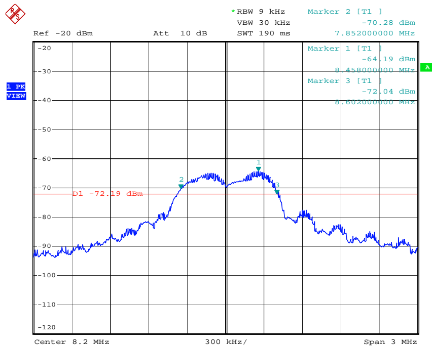
Figure 3: Spectral diagram, emission bandwidth measurement
