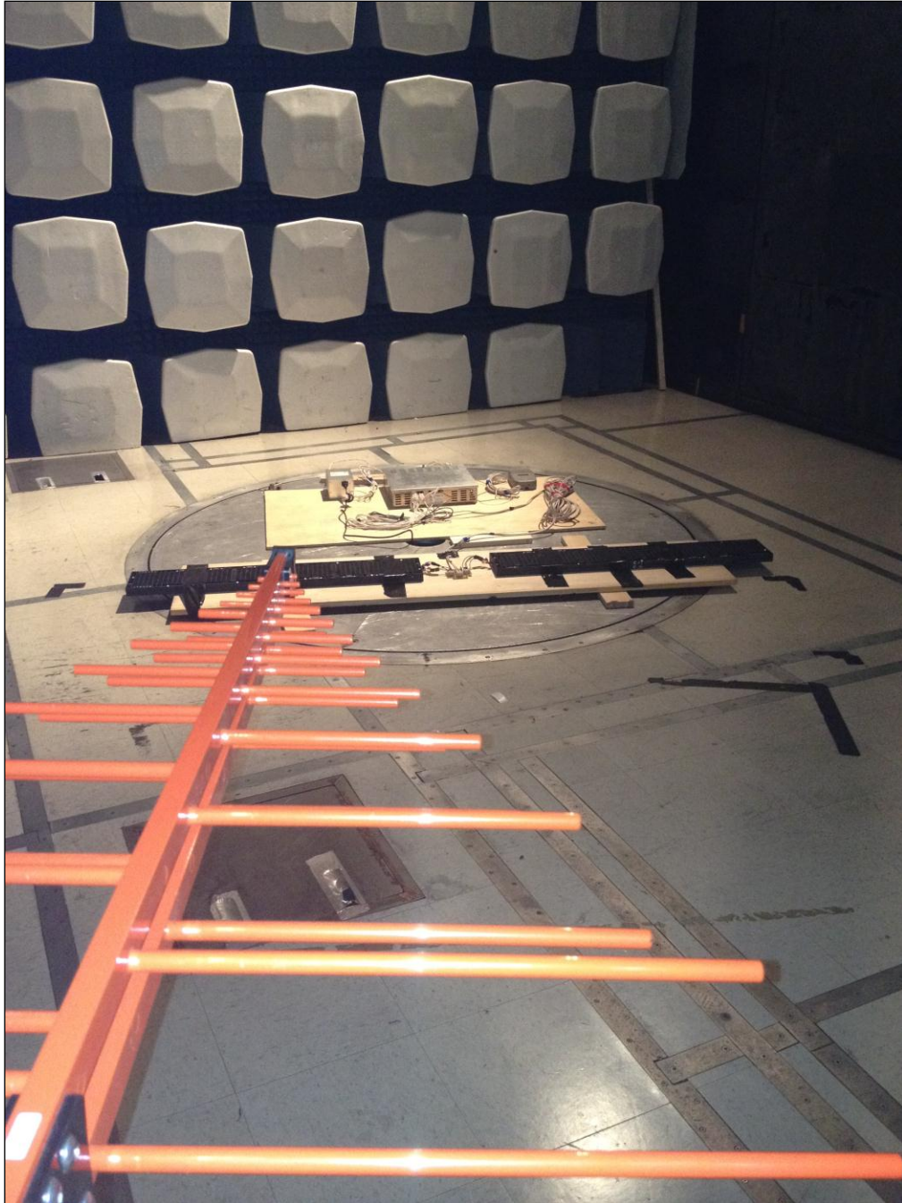
Photograph 5. Radiated Spurious Emissions, Test Setup
