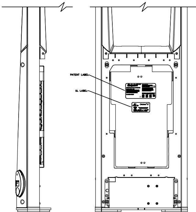
EVOLVE P20 REAR MOUNTING PANEL
