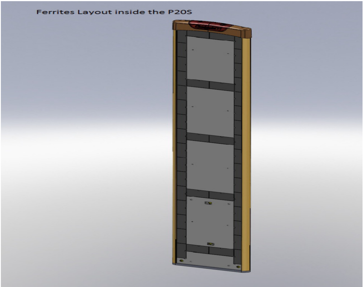
Figure 3: Ferrites layout inside the P20S
