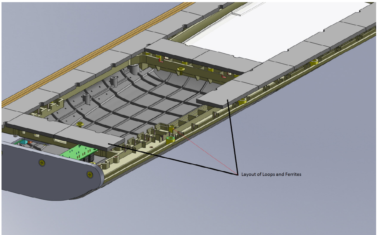
Figure 4: Layout of loops and ferrites inside P20S
