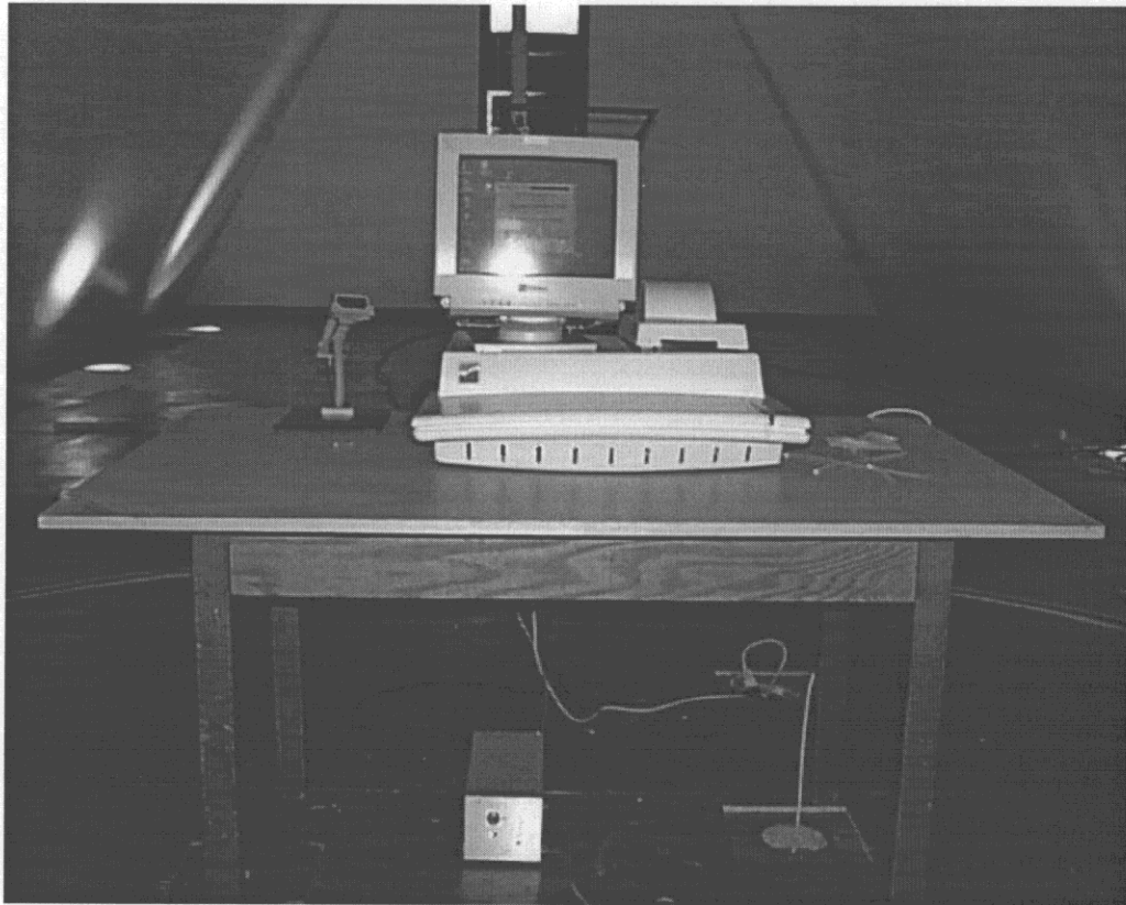
Checkstation Reader - Radiated EMI Test Setup
