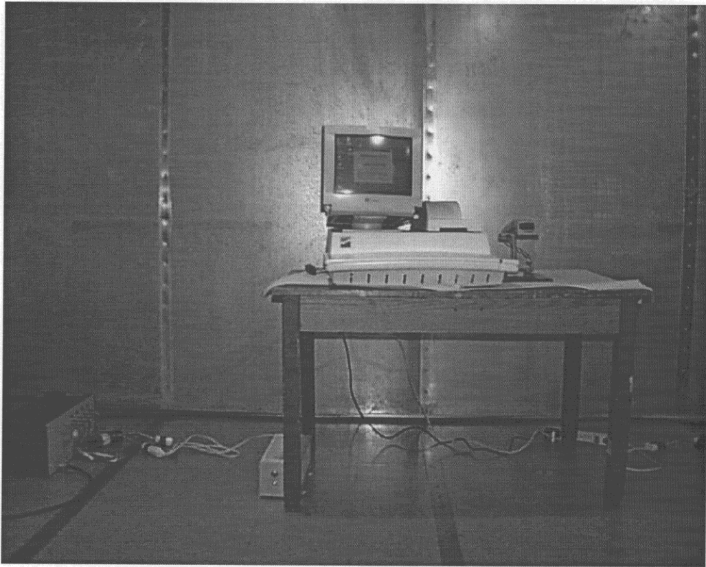
Checkstation Reader - Conducted EMI Test Setup
