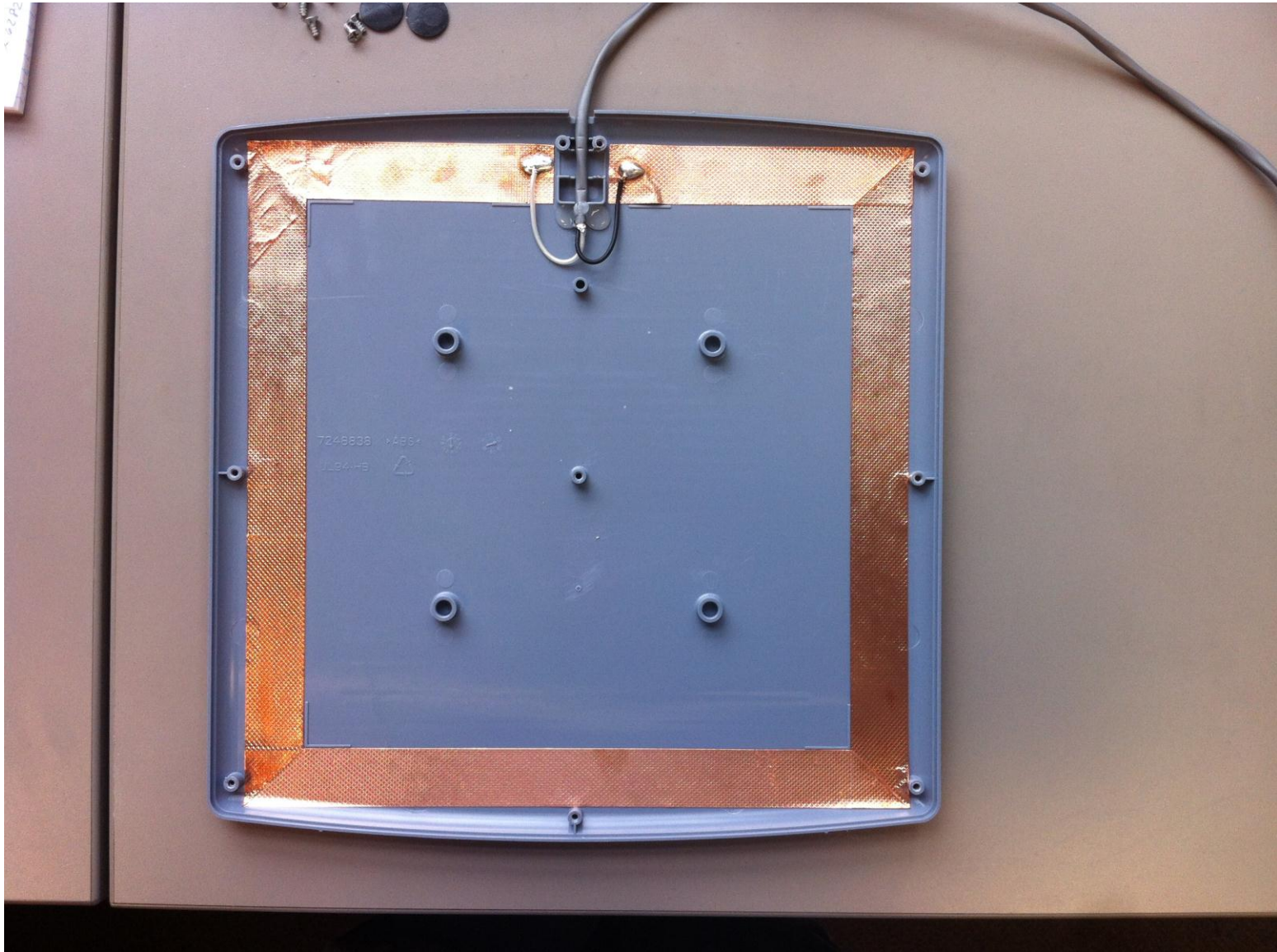
Antenna - Internal
