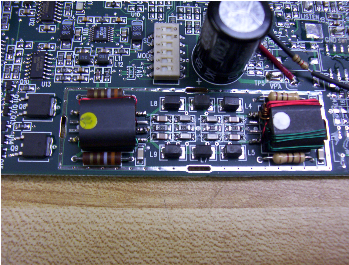
Checkpoint Systems, Inc.: Internal Photo of CP9-2 PCB, close-up of RF shielded area
