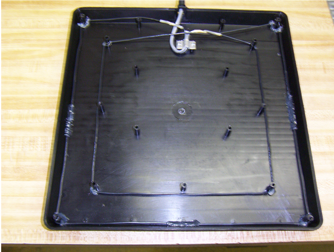
Checkpoint Systems, Inc.: Internal Photo of CP9-2 Antenna
