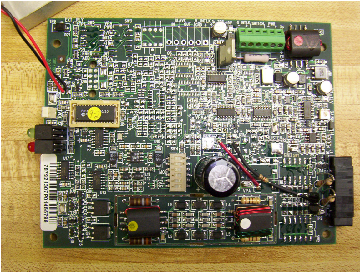
Checkpoint Systems, Inc.: Internal Photo of CP9-2 with RF shield removed
