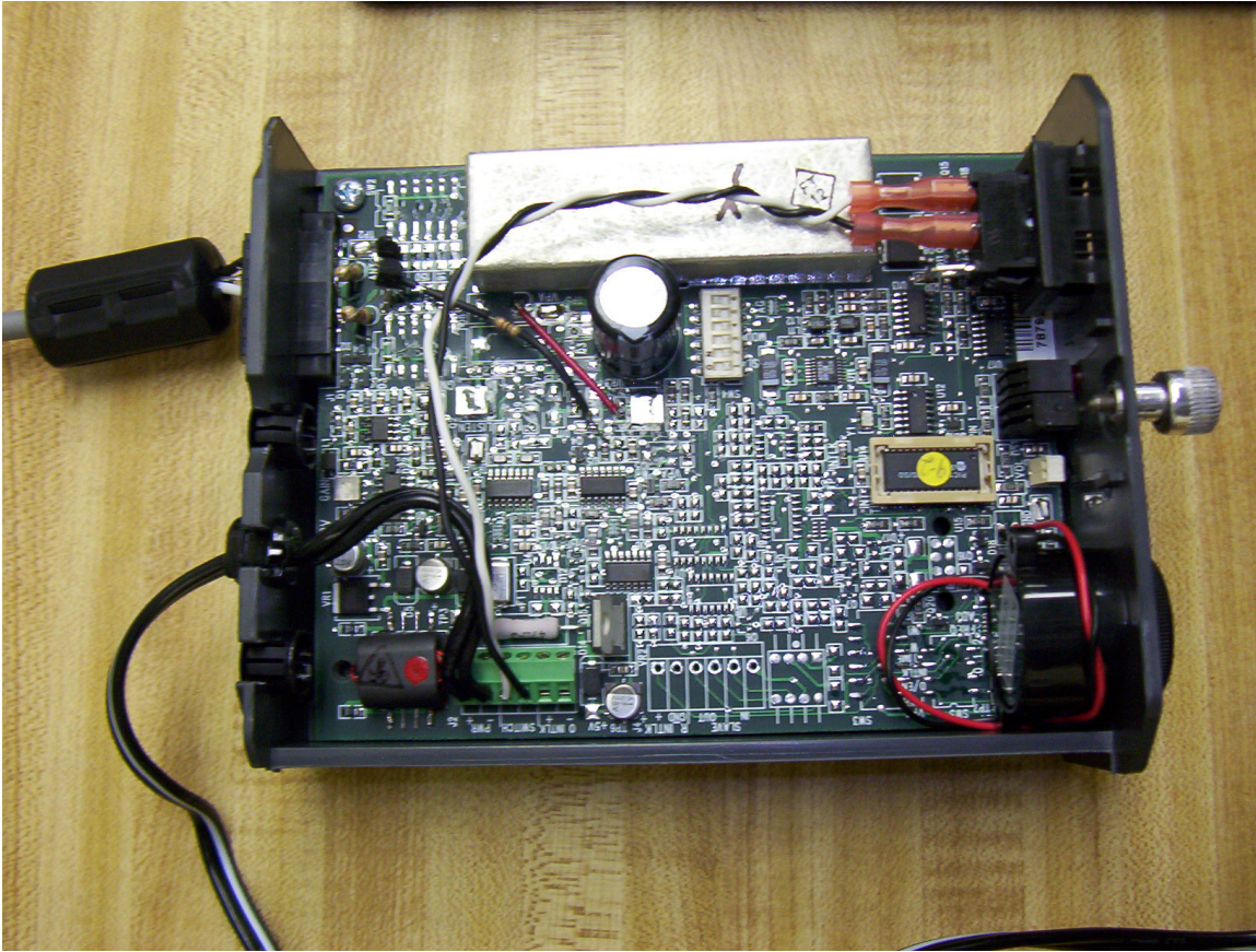
Checkpoint Systems, Inc.: Internal Photo of CP9-2 with cover removed
