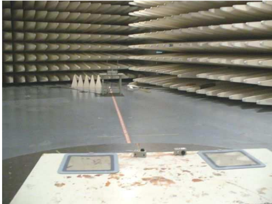
Photograph 4: Set-up for radiated emission (9kHz - 30MHz)
