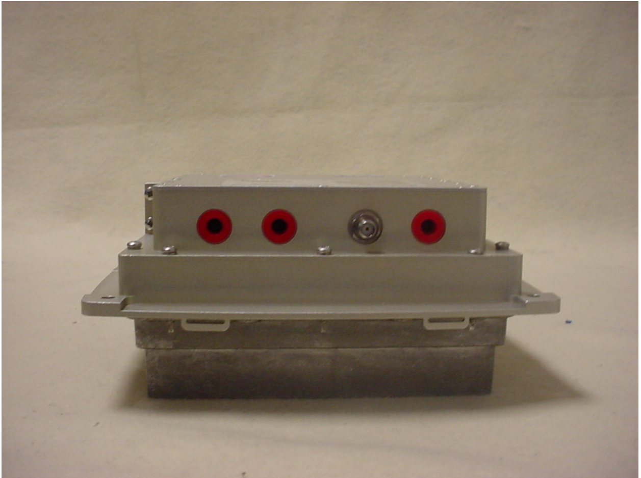
Figure 7: External – Side View without Radome cover
