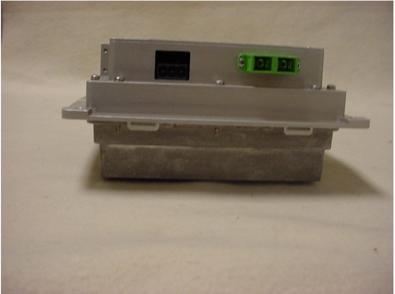
Figure 5: External – Side View without Radome cover
