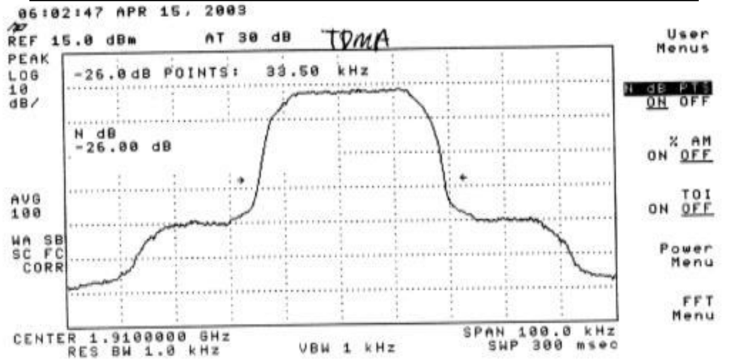
Plot 273: TDMA Mode Uplink - High Channel
