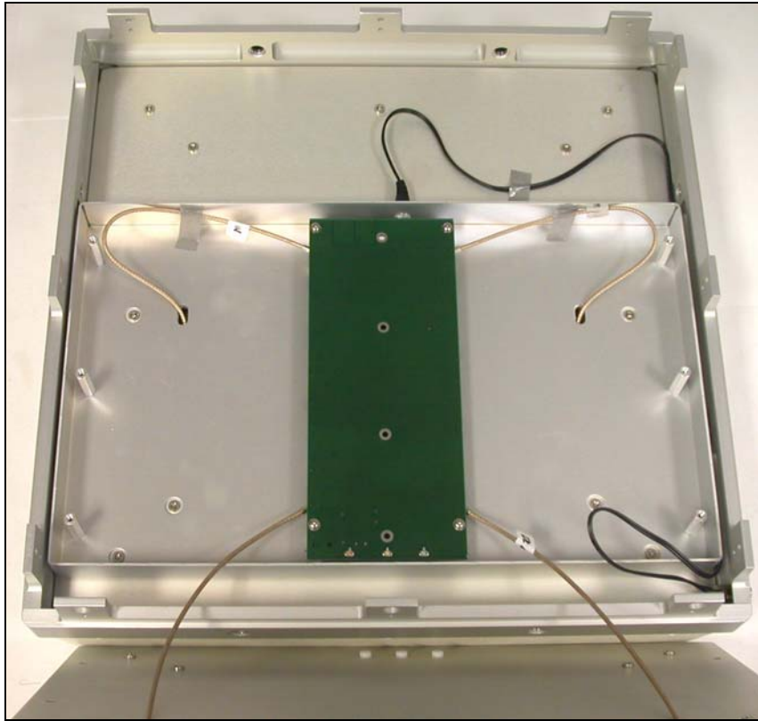
Figure 1: Internal – PCB Mounted In Enclosure
