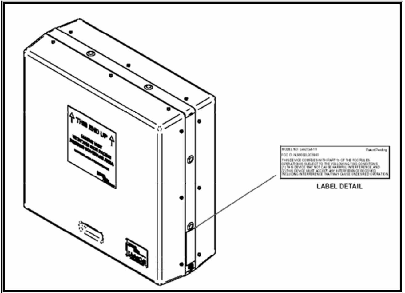
Figure G-2: Label Location Drawing
