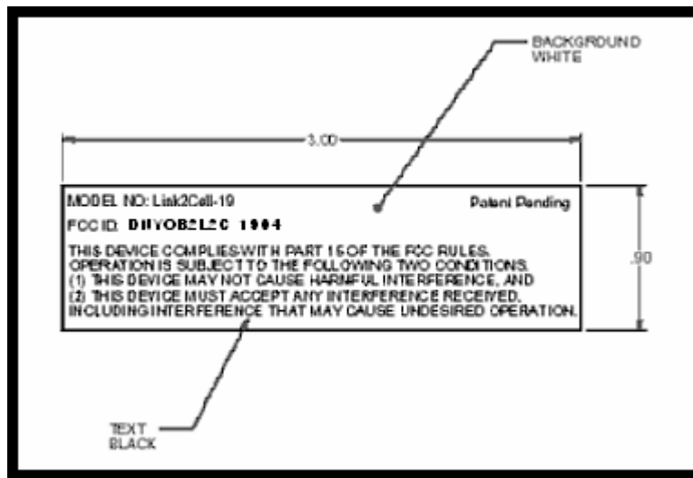
Figure G-1: Label Drawing
