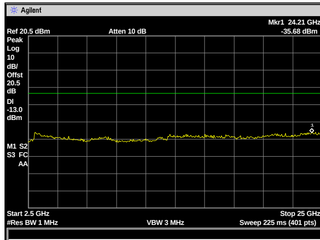
Figure 25: Spurious Emissions - CDMA High Channel – 2.5 to 25 GHz
