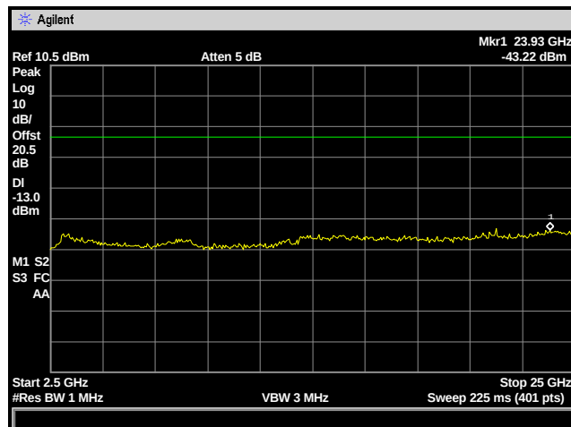
Figure 15: Spurious Emissions - TDMA Mid Channel – 2.5 to 25 GHz
