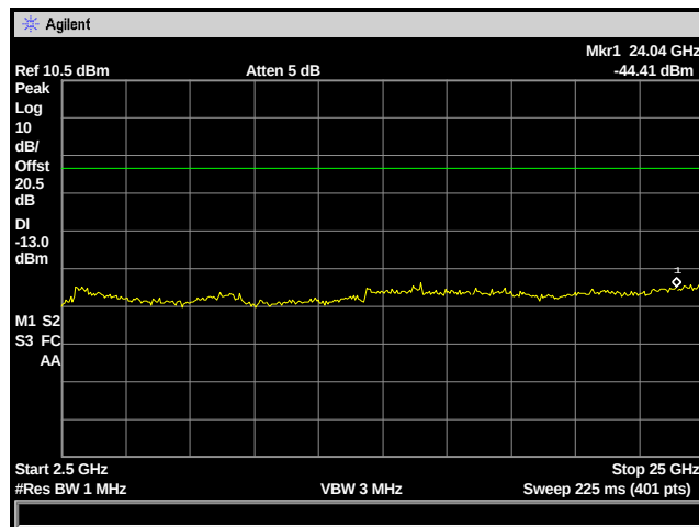
Figure 8: Spurious Emissions - CDMA Mid Channel – 2.5 to 25 GHz
