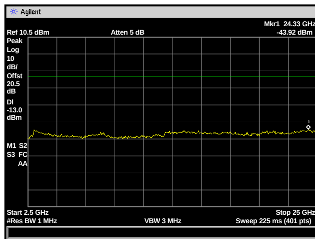
Figure 6: Spurious Emissions - CDMA Low Channel – 2.5 to 25 GHz
