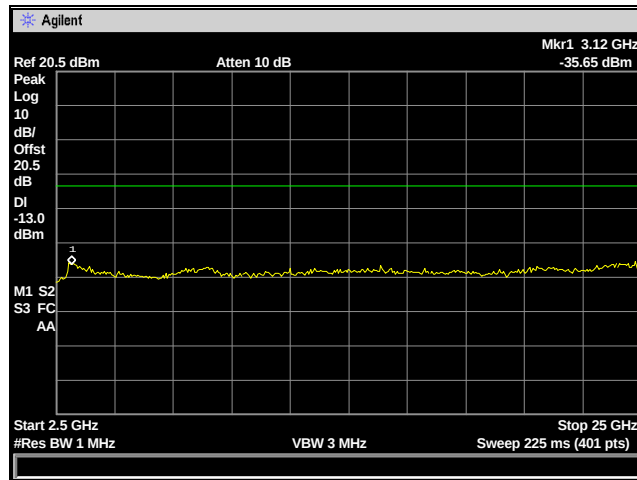
Figure 22: Spurious Emissions - GSM Low Channel – 2.5 to 25 GHz
