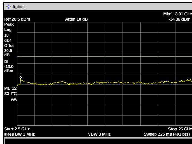
Figure 24: Spurious Emissions - GSM Mid Channel – 2.5 to 25 GHz
