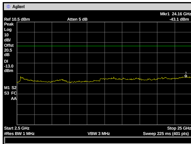
Figure 20: Spurious Emissions – CW Low Channel – 2.5 to 25 GHz
