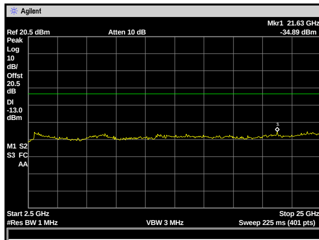
Figure 17: Spurious Emissions - TDMA High Channel – 2.5 to 25 GHz
