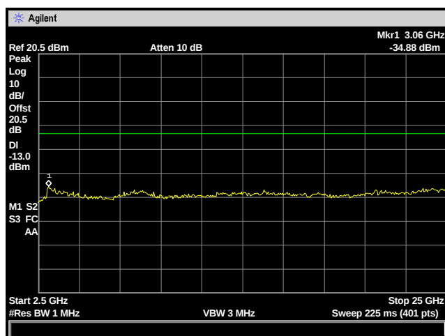
Figure 26: Spurious Emissions - GSM High Channel – 2.5 to 25 GHz
