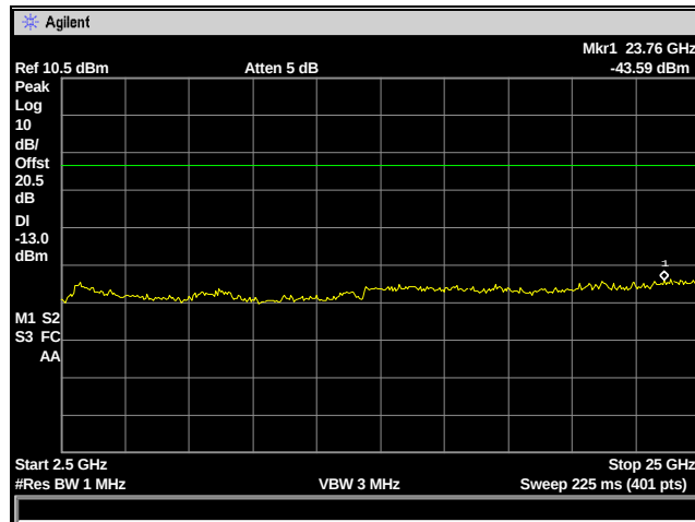
Figure 13: Spurious Emissions - TDMA Low Channel – 2.5 to 25 GHz
