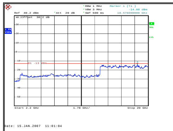
Figure 14: Spurious Emissions - Downlink CDMA Mid Channel – 2.2 to 20 GHz
