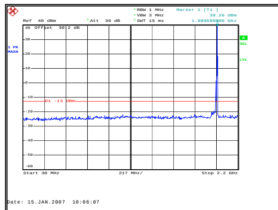
Figure 36: Spurious Emissions - Downlink GSM High Channel – 30 MHz to 2.2 GHz
