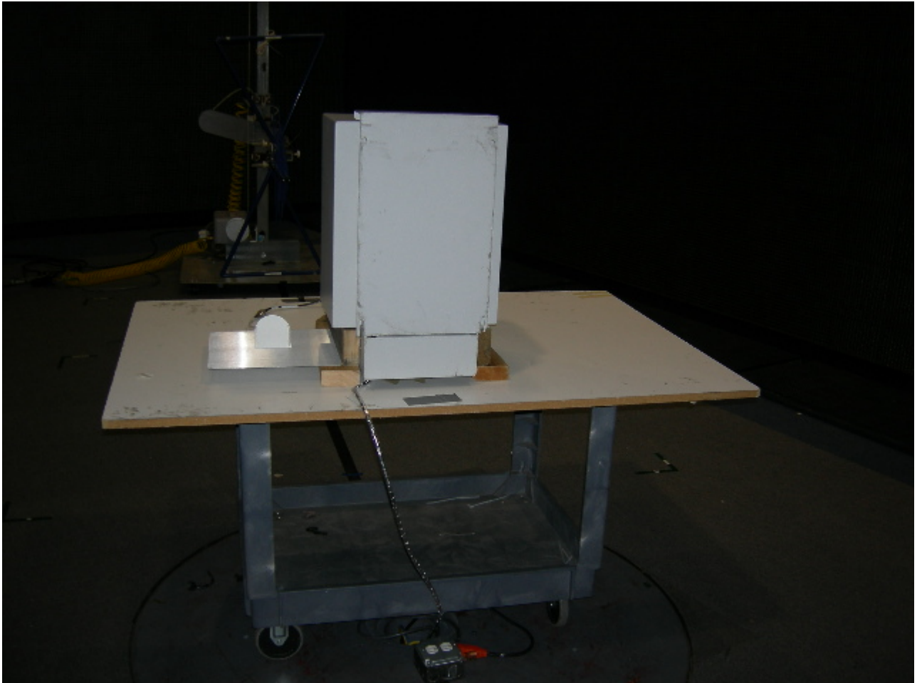
Figure 4: Test Setup - Radiated Emissions - Unintentional
