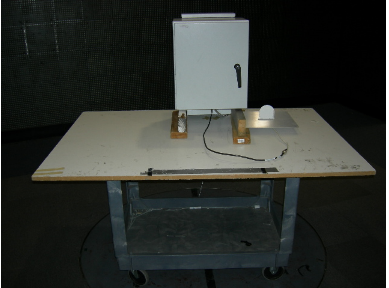
Figure 3: Test Setup – Radiated Emissions - Unintentional
