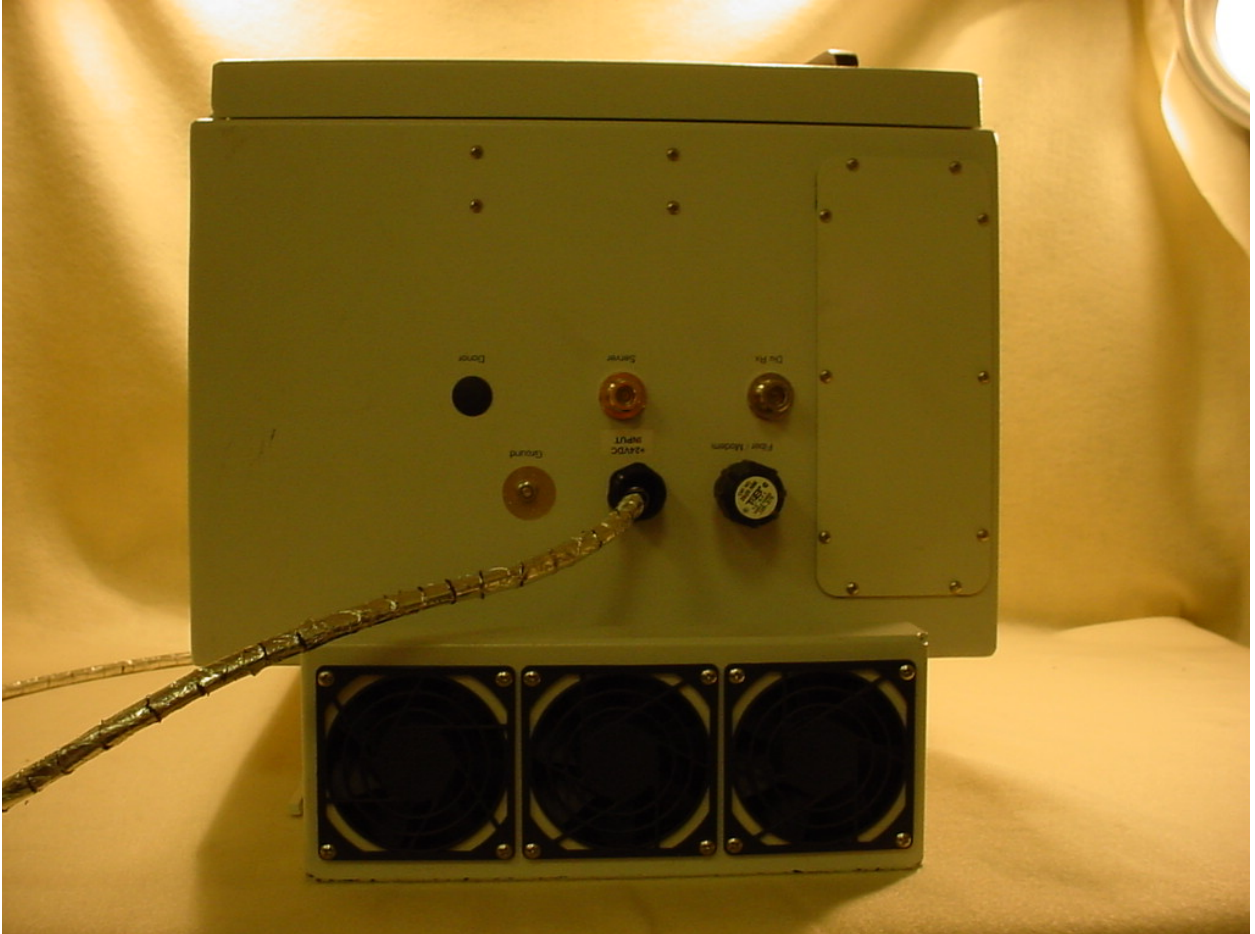
Figure 3: External – Bottom
