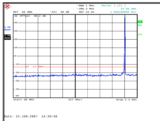
Figure 30: Spurious Emissions - Downlink CW High Channel – Inter-modulation - 30 MHz to 2.2 GHz
