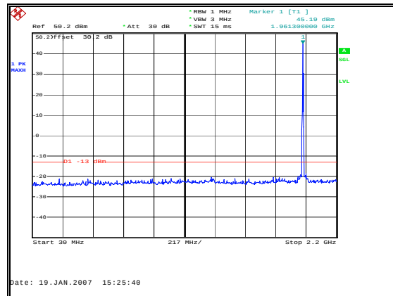
Figure 21: Spurious Emissions - Downlink TDMA Mid Channel – 30 MHz to 2.2 GHz
