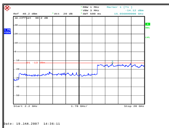
Figure 14: Spurious Emissions - Downlink CDMA Mid Channel – 2.2 to 20 GHz
