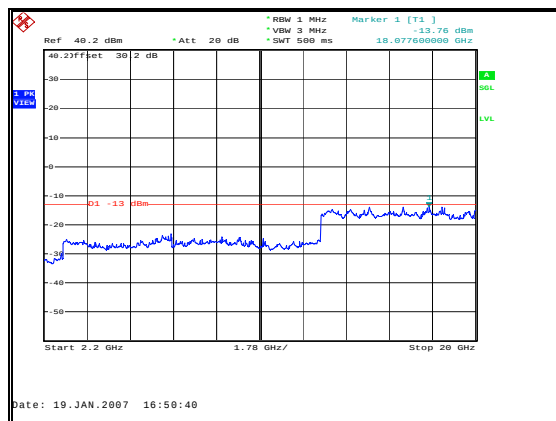
Figure 12: Spurious Emissions - Downlink CDMA Low Channel – Inter-modulation – 2.2 to 20 GHz
