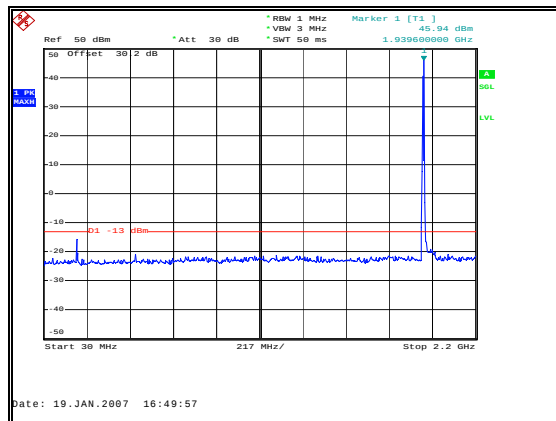
Figure 11: Spurious Emissions - Downlink CDMA Low Channel – Inter-modulation-30MHz to 2.2GHz
