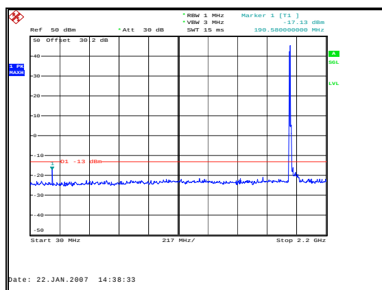
Figure 27: Spurious Emissions - Downlink CW Low Channel – Inter-modulation - 30 MHz to 2.2 GHz
