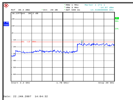
Figure 20: Spurious Emissions - Downlink TDMA Low Channel – Inter-modulation – 2.2 to 20 GHz
