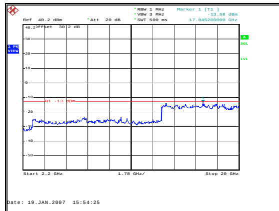
Figure 37: Spurious Emissions - Downlink GSM High Channel – 2.2 to 20 GHz
