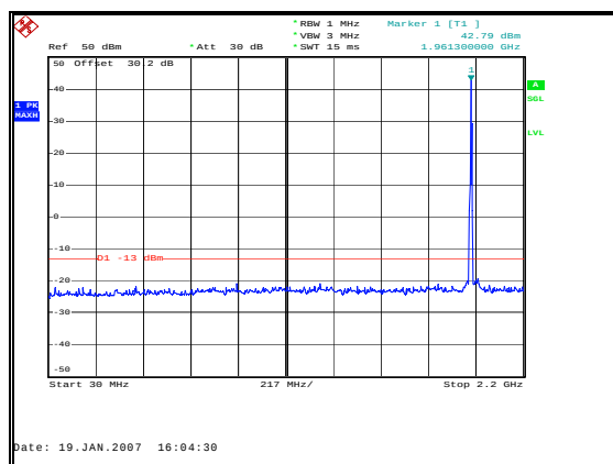
Figure 34: Spurious Emissions - Downlink GSM Mid Channel – 30 MHz to 2.2 GHz
