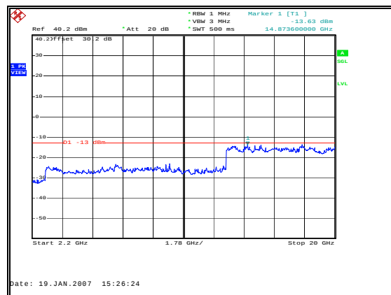
Figure 22: Spurious Emissions - Downlink TDMA Mid Channel – 2.2 to 20 GHz
