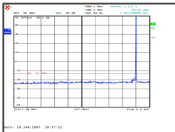
Figure 16: Spurious Emissions - Downlink CDMA High Channel –Inter-modulation-30MHz to 2.2GHz
