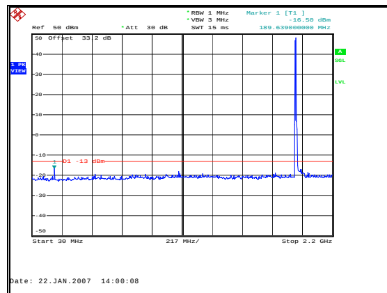
Figure 19: Spurious Emissions - Downlink TDMA Low Channel – Inter-modulation-30MHz to 2.2GHz
