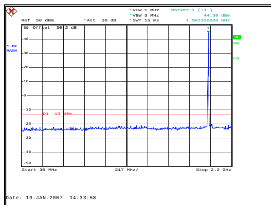
Figure 13: Spurious Emissions - Downlink CDMA Mid Channel – 30 MHz to 2.2 GHz
