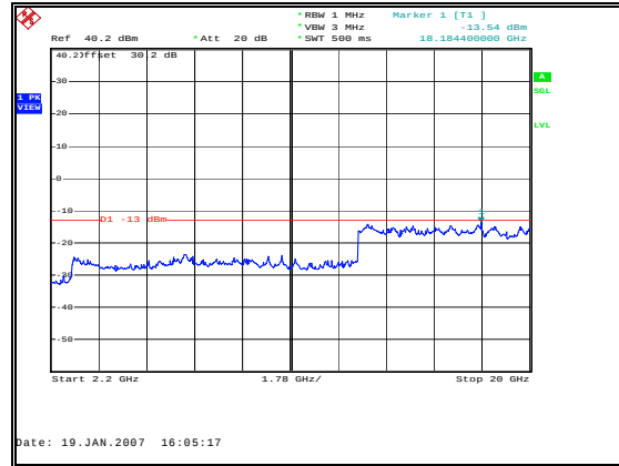
Figure 35: Spurious Emissions - Downlink GSM Mid Channel – 2.2 to 20 GHz
