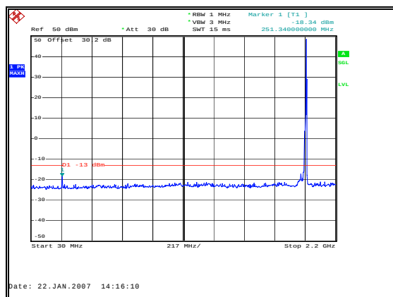
Figure 24: Spurious Emissions - Downlink TDMA High Channel –Inter-modulation-30MHz to 2.2GHz
