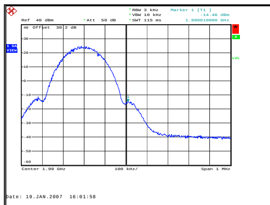
Figure 43: Band-Edge Downlink GSM High Channel
