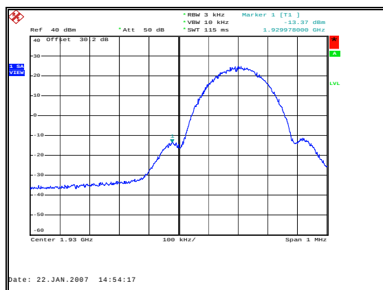
Figure 42: Band-Edge Downlink GSM Low Channel
