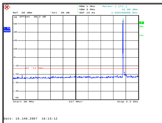
Figure 32: Spurious Emissions - Downlink GSM Low Channel – 30 MHz to 2.2 GHz
