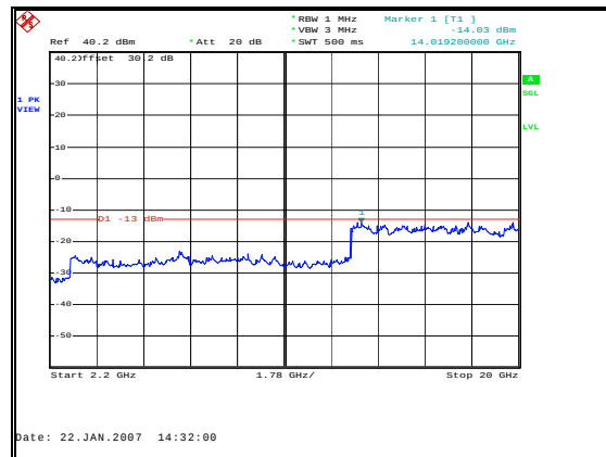
Figure 31: Spurious Emissions - Downlink CW High Channel – Inter-modulation – 2.2 to 20 GHz
