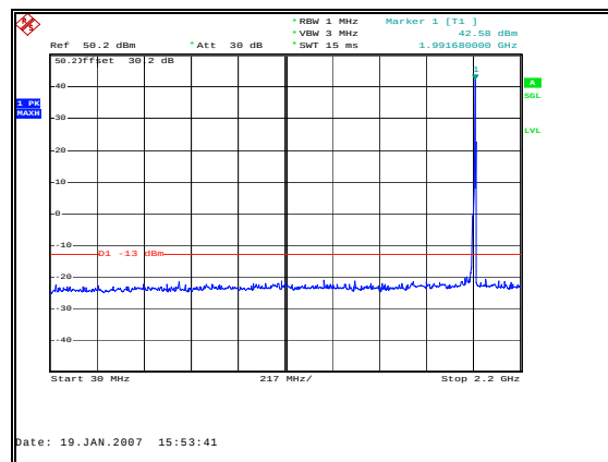
Figure 36: Spurious Emissions - Downlink GSM High Channel – 30 MHz to 2.2 GHz
