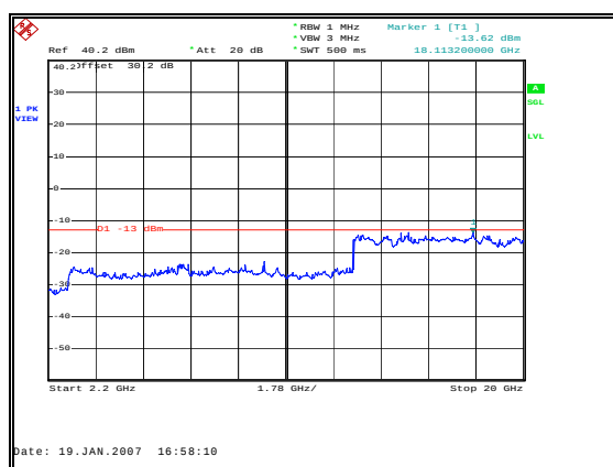
Figure 17: Spurious Emissions - Downlink CDMA High Channel – Inter-modulation – 2.2 to 20 GHz
