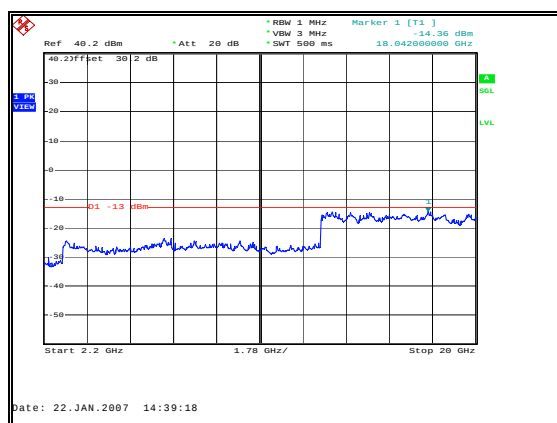
Figure 28: Spurious Emissions - Downlink CW Low Channel – Inter-modulation – 2.2 to 20 GHz
