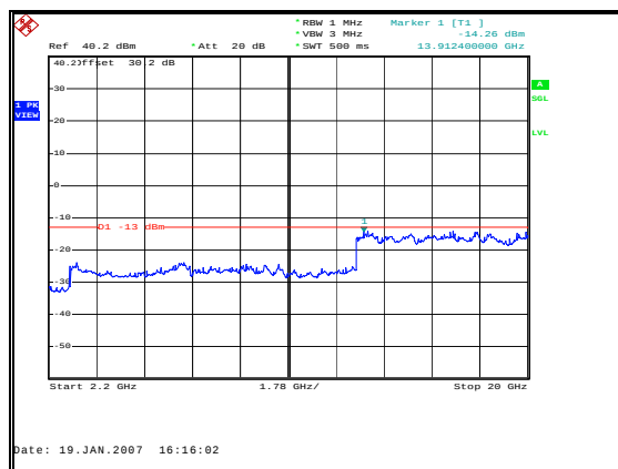
Figure 33: Spurious Emissions - Downlink GSM Low Channel – 2.2 to 20 GHz
