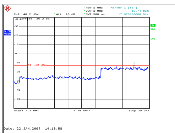
Figure 25: Spurious Emissions - Downlink TDMA High Channel – Inter-modulation – 2.2 to 20 GHz
